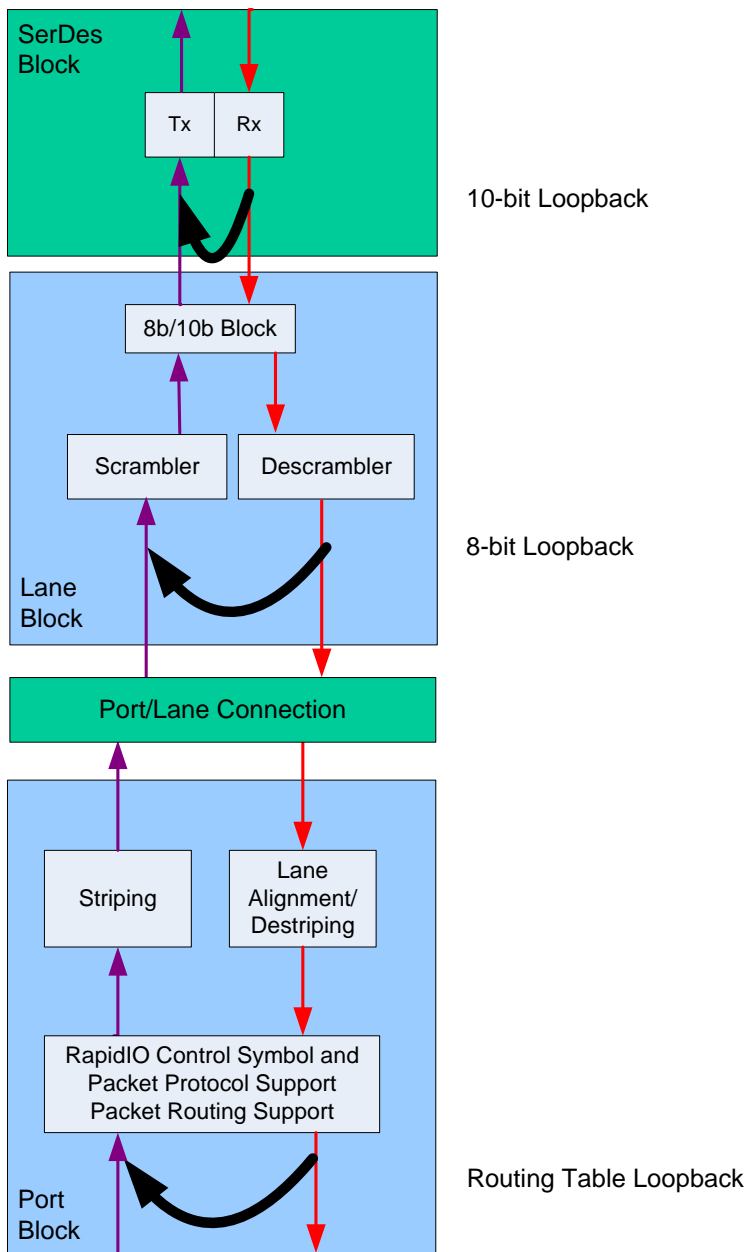
Figure 14: Loopback Locations
