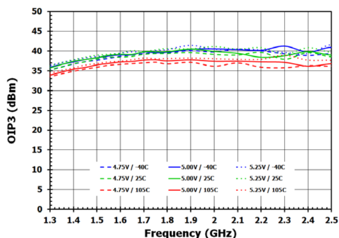
Figure 11: OIP3
