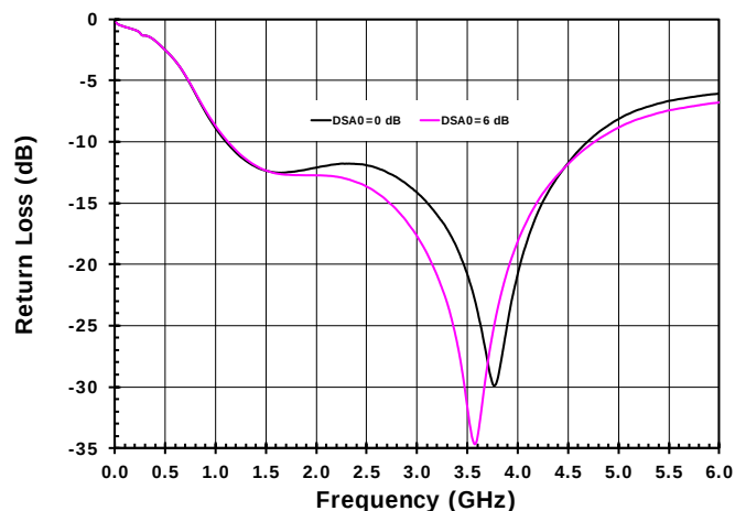
Figure 9. Output Return Loss for DSA0 Settings
