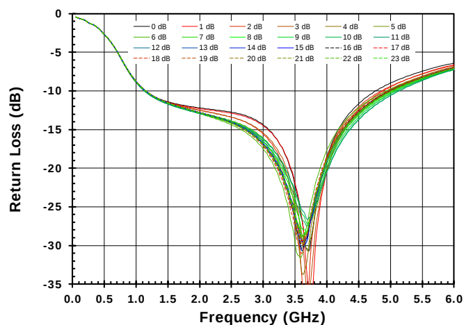
Figure 11. Output Return Loss for DSA1 Settings
