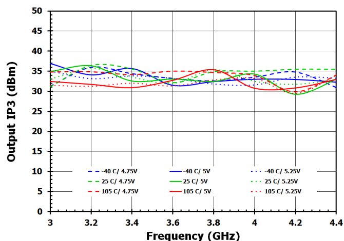
Figure 62. OIP3 vs. Frequency with P_{OUT} = -10\text{dBm/Tone} and Max Gain
