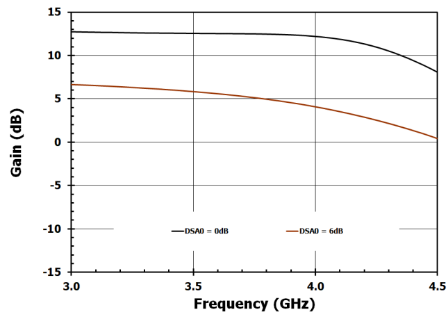
Figure 38. Gain vs. Frequency for DSA0 Settings
