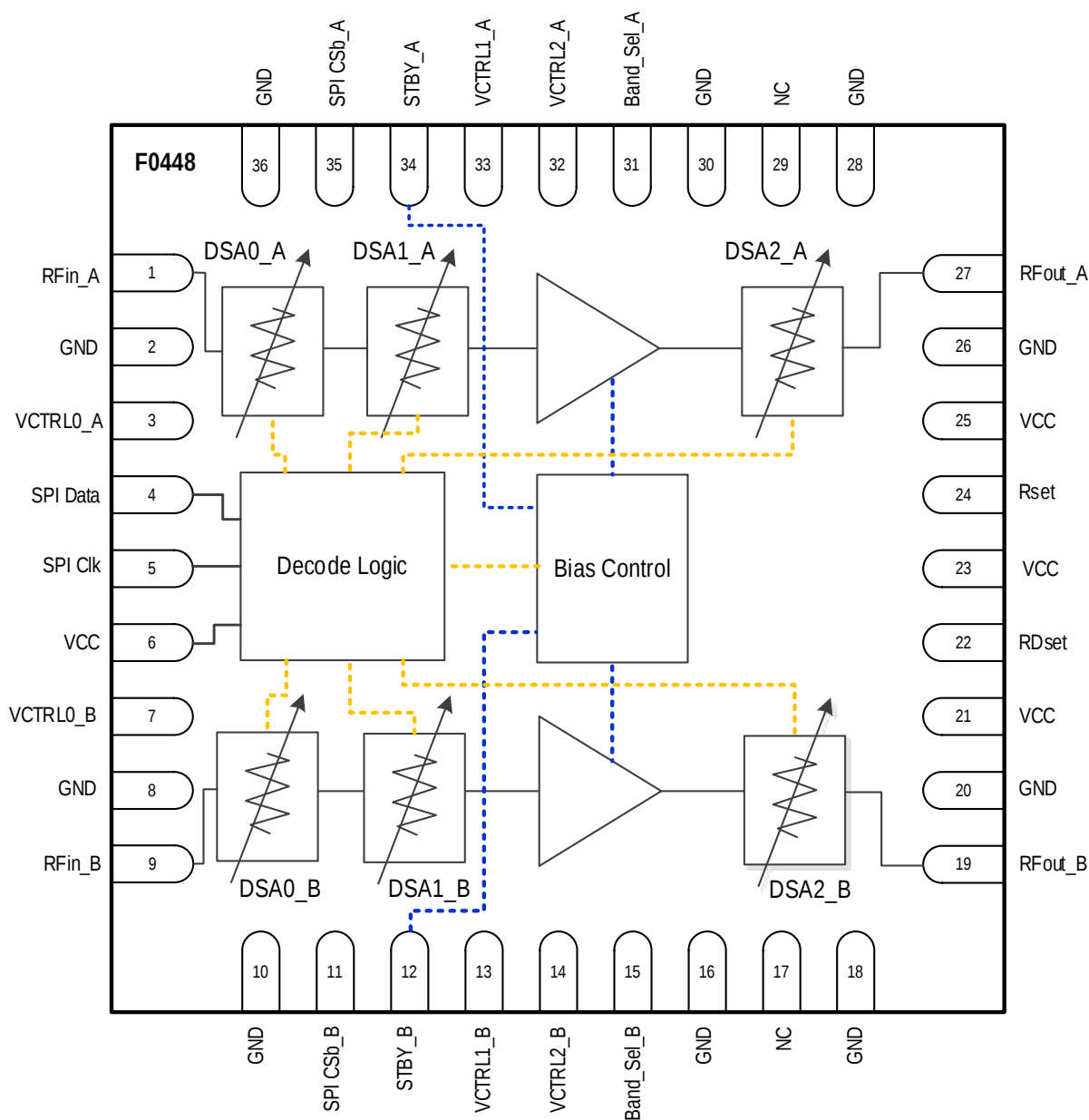
Figure 2. Pin Assignments – Top View
