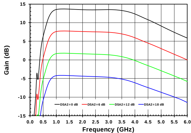
Figure 6. Gain vs. Frequency for DSA2 Settings
