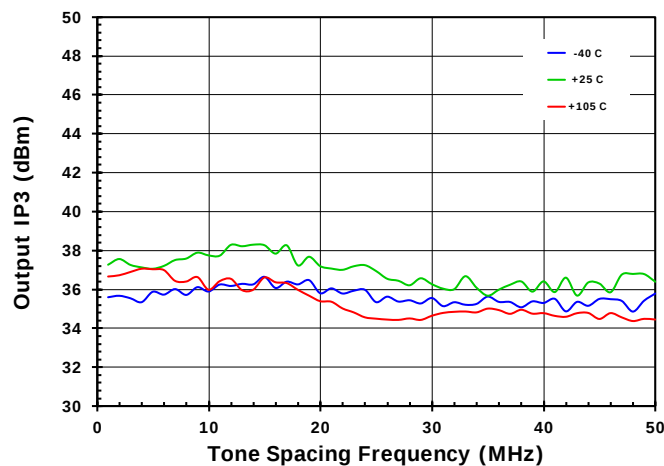
Figure 29. OIP3 vs. Frequency as a Function of Tone Spacing with P_{OUT} = 0\text{dBm/Tone} at 3.6GHz
