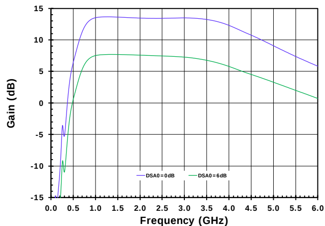
Figure 4. Gain vs. Frequency for DSA0 Settings
