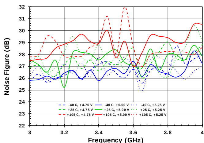
Figure 34. NF vs. Frequency as a Function of Temperature with DSA1 = 22dB
