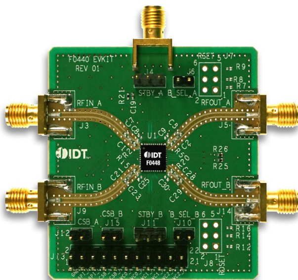
Figure 72. Evaluation Board – Top View
