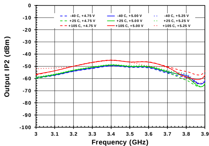
Figure 32. Wideband OIP2 vs. Frequency with P_{OUT} = 0\text{dBm/Tone}
