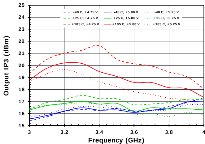
Figure 30. OIP3 vs. Frequency with P_{OUT} = 0\text{dBm/Tone} and DSA0 = 6dB
