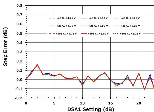
Figure 23. DSA1 Attenuator Step Error (DNL) at 3.6GHz
