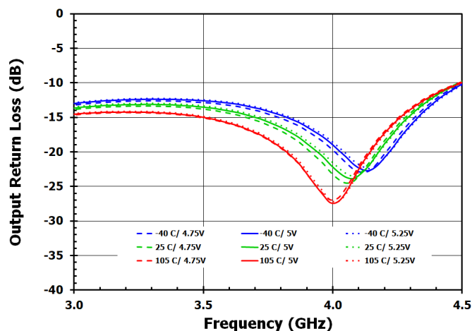
Figure 42. Output Return Loss vs. Frequency
