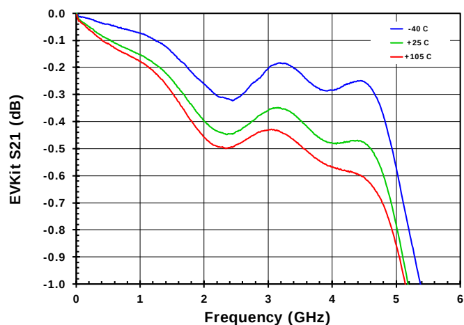
Figure 36. EVKit Connector and Trace Losses
