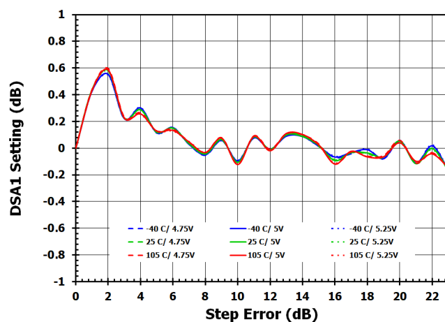
Figure 58. DSA1 Attenuator Step Error (DNL) at 4GHz
