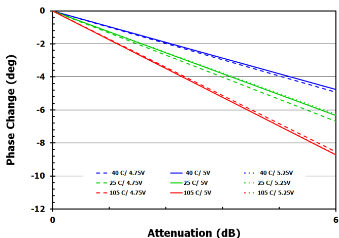
Figure 50. Phase Deviation Between Adjacent States vs. DSA0 Setting (4GHz)
