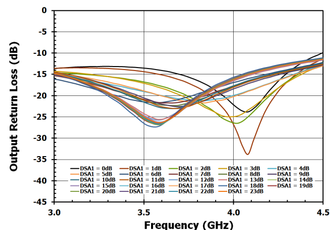
Figure 46. Output Return Loss for DSA1 Settings
