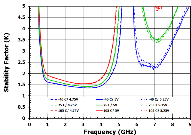
Figure 66. Stability Factor (K)
