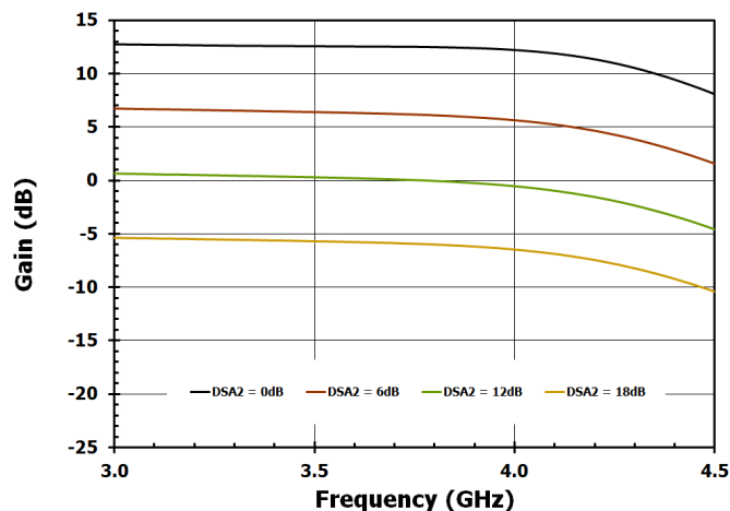
Figure 40. Gain vs. Frequency for DSA2 Settings
