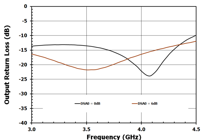
Figure 44. Output Return Loss for DSA0 Settings
