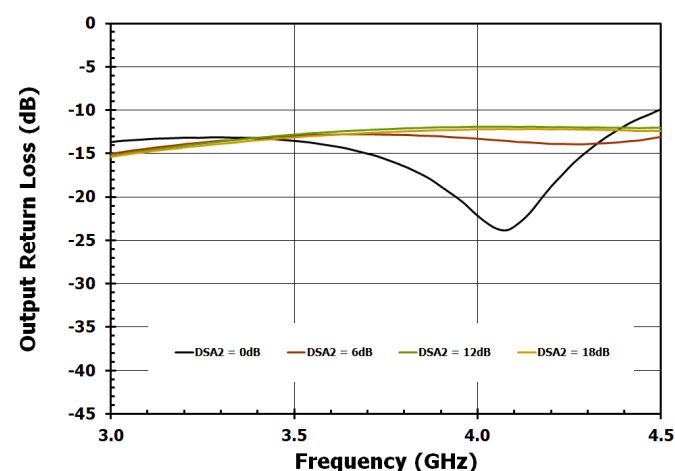
Figure 48. Output Return Loss for DSA2 Settings
