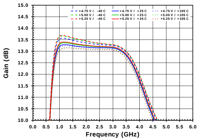
Figure 3. Maximum Gain vs. Frequency
