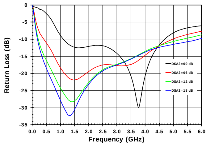
Figure 13. Output Return Loss for DSA2 Settings
