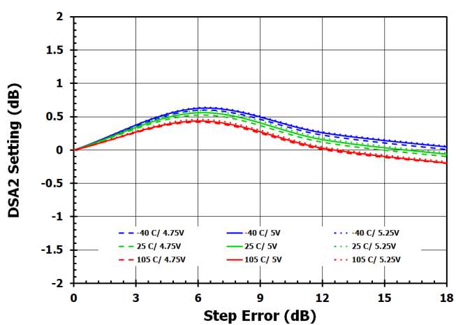
Figure 60. DSA2 Attenuator Step Error (DNL) at 4GHz
