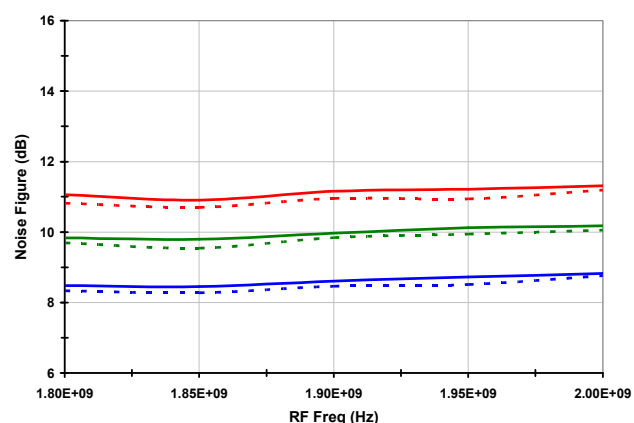
Noise Figure ChA vs. ChB
