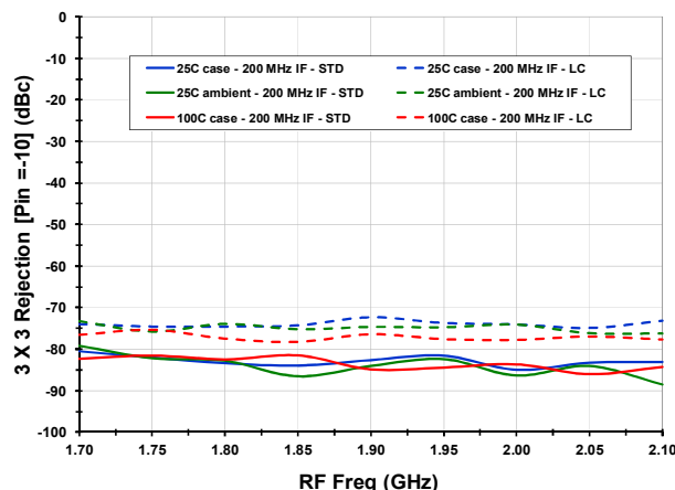
3RF x 3LO rejection
