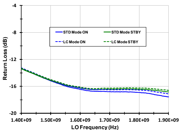
EVKit LO Port Match ( T_A = 25^\circ\text{C} , P_{MEAS} = 0\text{ dBm} )
