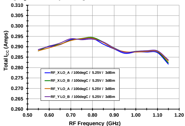
I_{CC} [ High Side Injection ]
