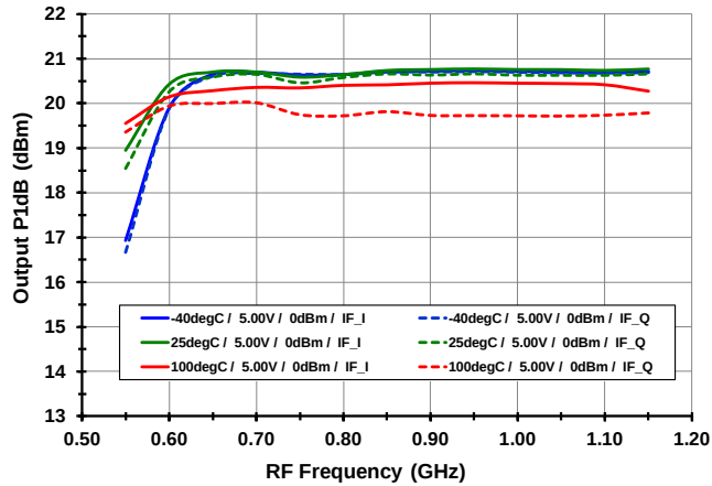
P1dB O vs. T CASE [ Low Side Injection ]
