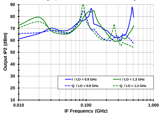
IP2 o Flatness [High Side Injection, RF_X LO_A]
