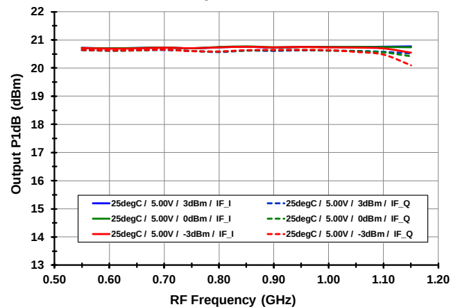
P1dB O vs. LO level [ High Side Injection ]
