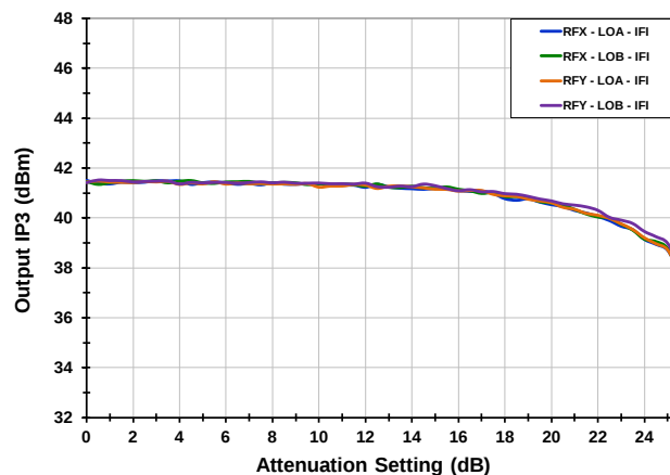
IP3 O [1.0 GHz RF, HiSide Inj.]
