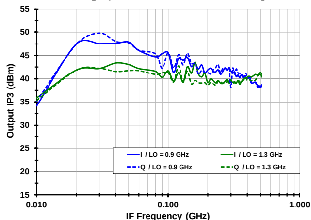
IP3 o Flatness [High Side Injection, RF_Y LO_B]
