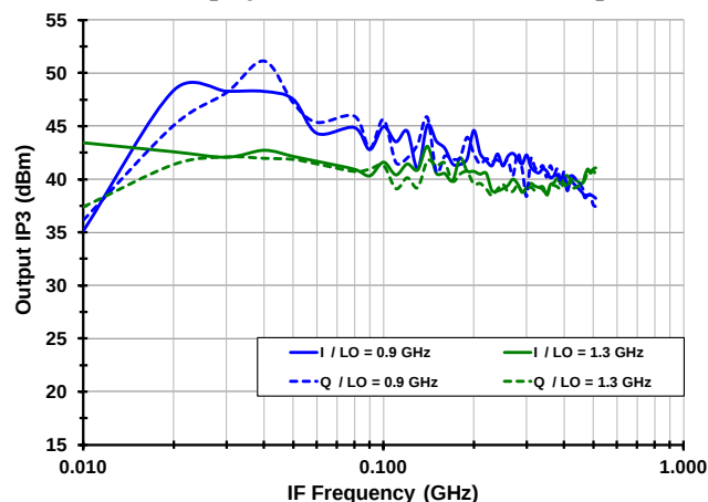
IP3 o Flatness [High Side Injection, RF_X LO_A]
