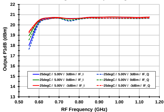
P1dB O vs. LO level [ Low Side Injection ]
