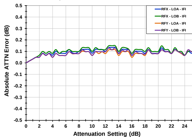
ATTN Accuracy [1.0 GHz RF, HiSide Inj.]
