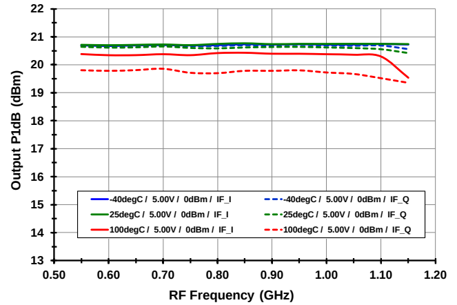
P1dB O vs. T CASE [ High Side Injection ]
