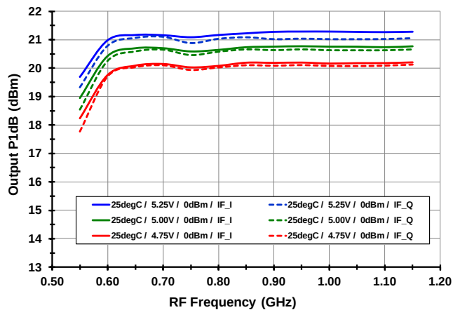
P1dB O vs. V CC [ Low Side Injection ]
