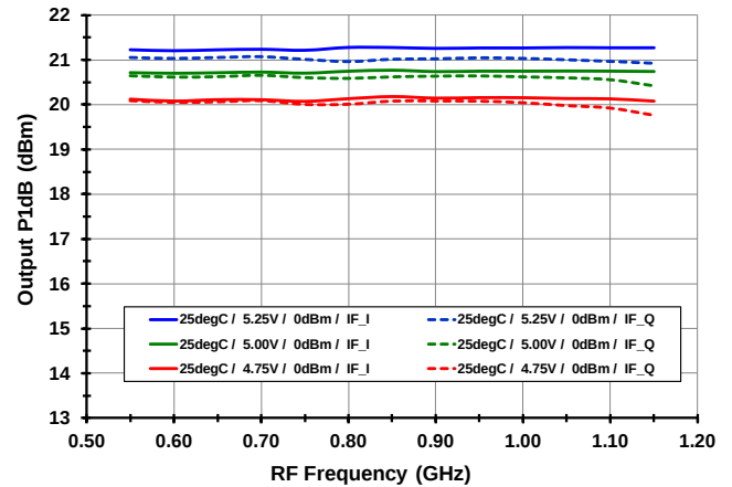
P1dB O vs. V CC [ High Side Injection ]
