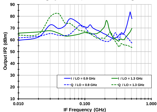
IP2 o Flatness [High Side Injection, RF_Y LO_B]
