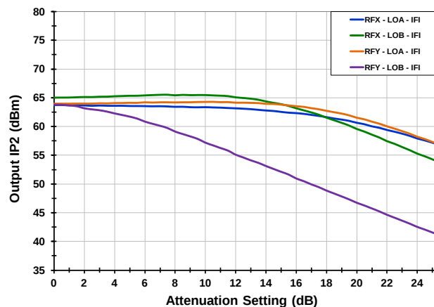
IP2 O [1.0 GHz RF, HiSide Inj.]
