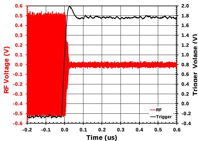
Figure 42. Switching Speed 0.0 to 31.5 dB
