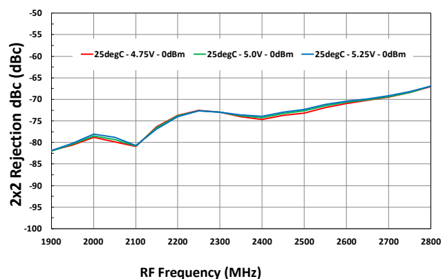
2x2 Rejection vs. V CC
