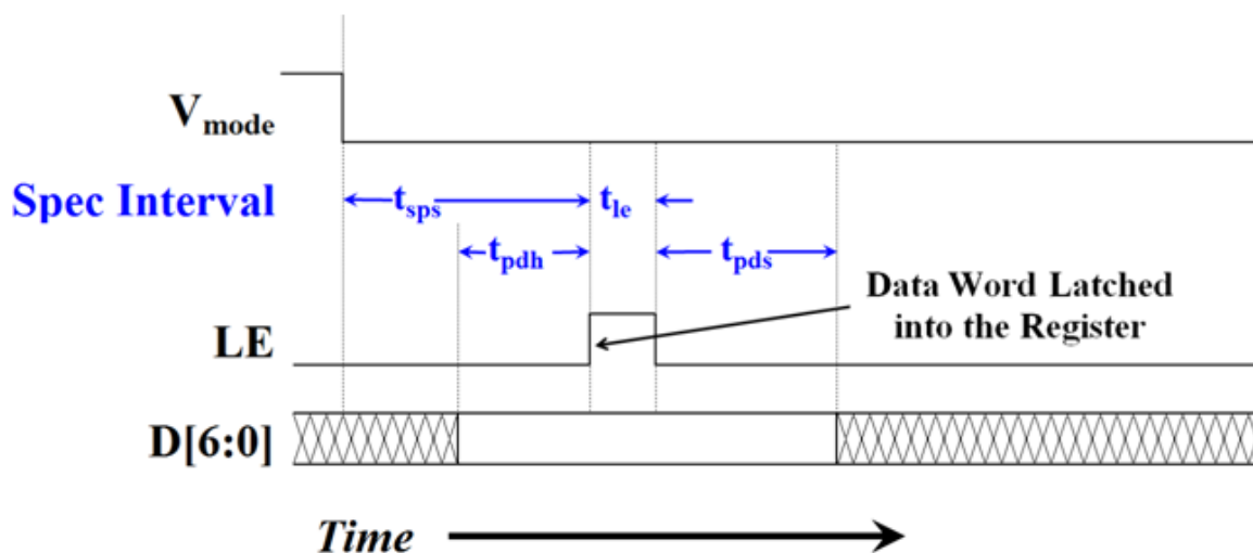
Figure 5. Latched Parallel Mode Timing Diagram
