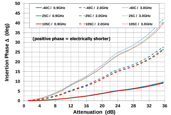
Insertion Phase \Delta vs. Attenuation
