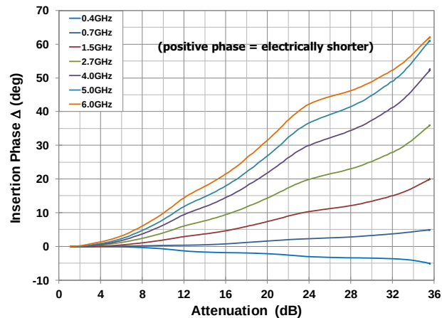
Insertion Phase \Delta vs. Attenuation
