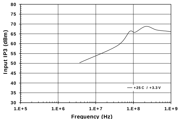
Figure 30. Input IP3
