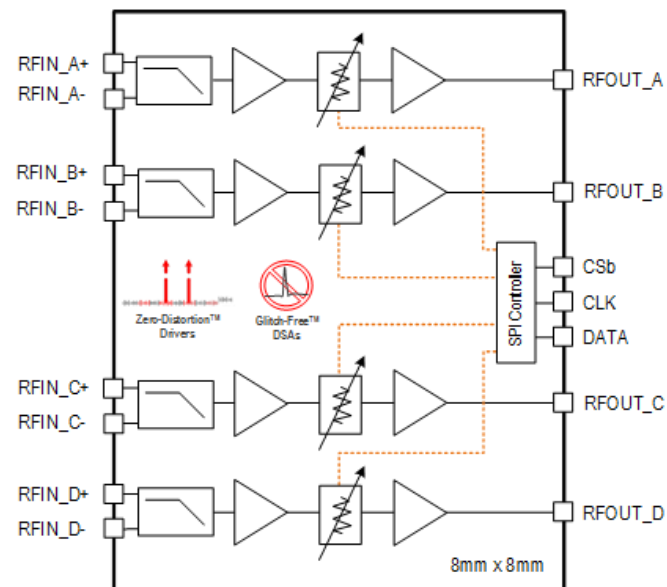
Figure 1. Block Diagram
