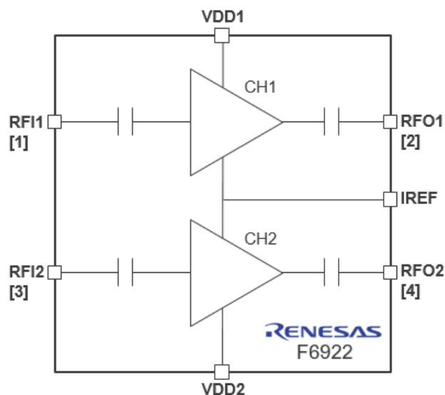
Figure 1. Block Diagram
