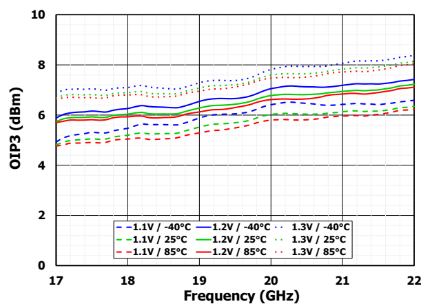
Figure 9. Output 3 rd Order Intercept
