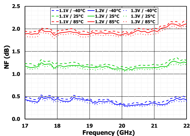
Figure 5. Noise Figure
