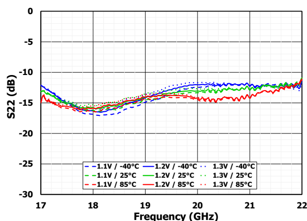
Figure 7. Output Match
