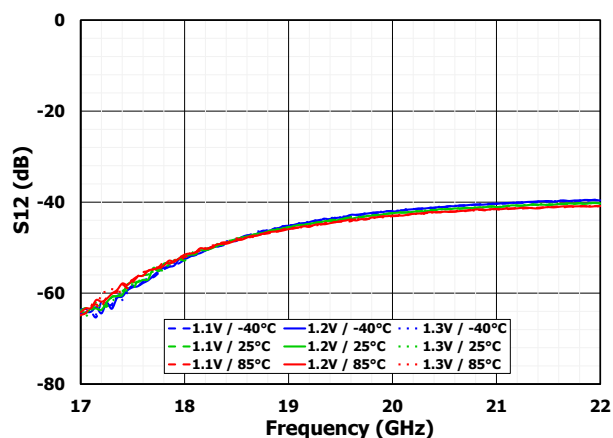
Figure 10. Reverse Isolation
