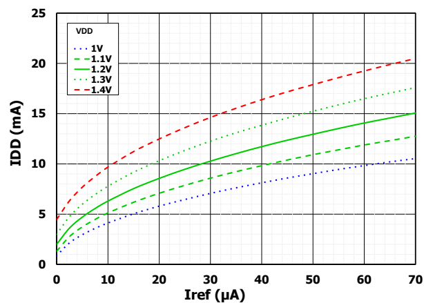
Figure 15. Supply Current vs Bias, Per Channel
