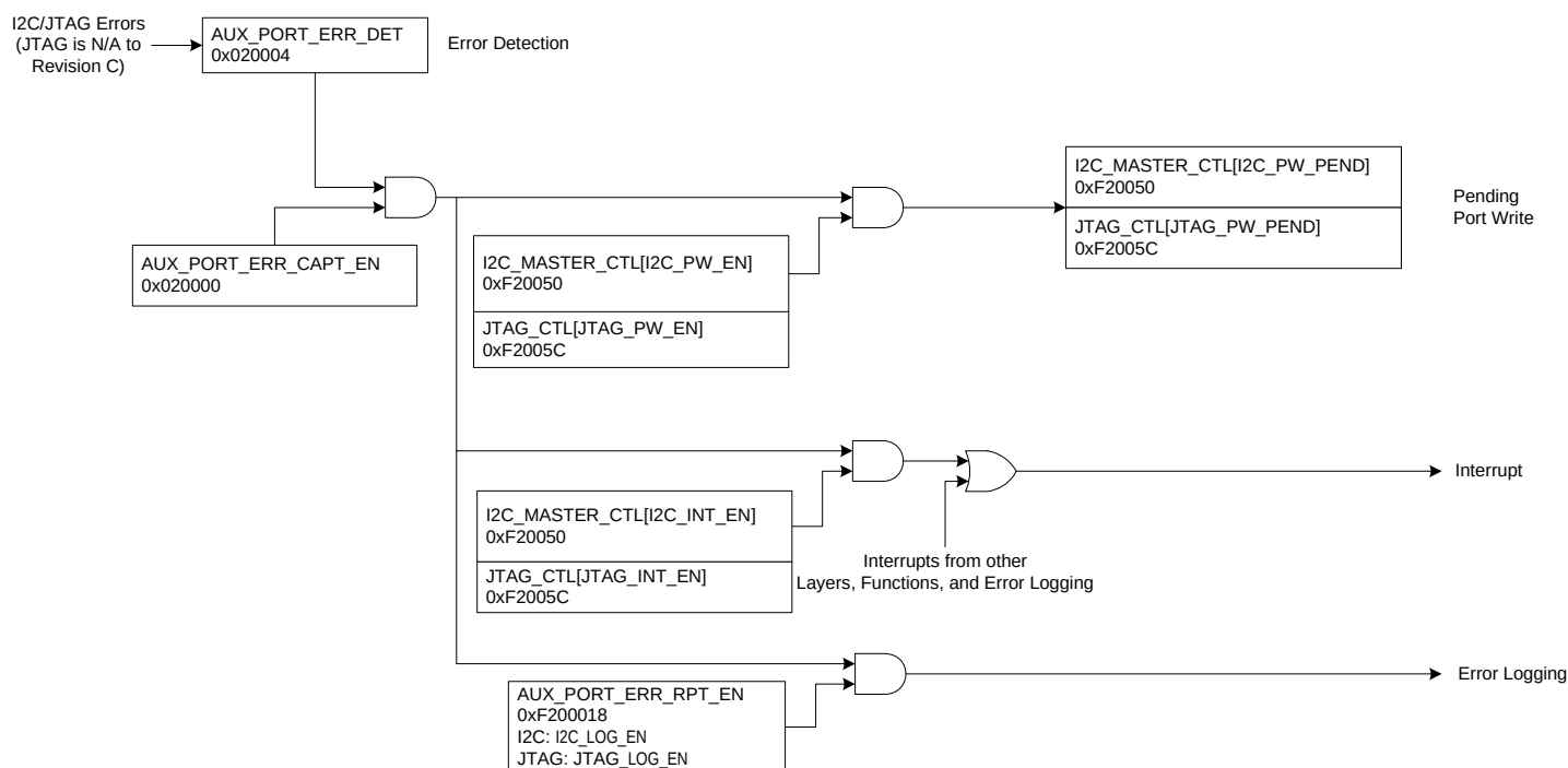
Figure 23: I 2 C Error Management Programming Model Flow Chart
