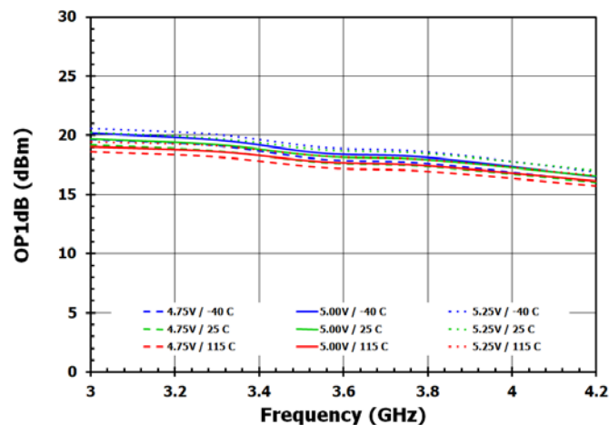
Figure 8. Output P1dB
