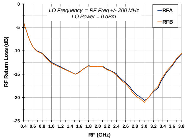
RF Port Return Loss vs. LO Frequency
