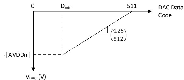
Figure 5. DAC Output Voltage vs 9-bit DAC Data
