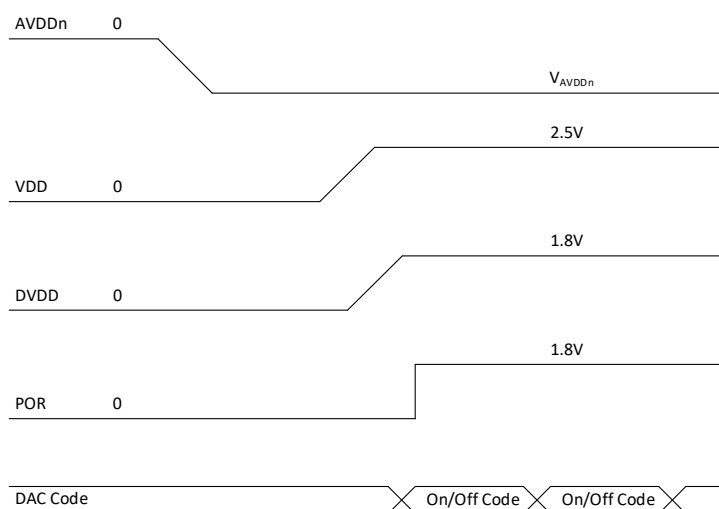
Figure 4. Recommended Power Sequence
