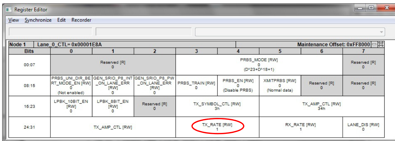
Figure 11: LANE_n_CTL Register
