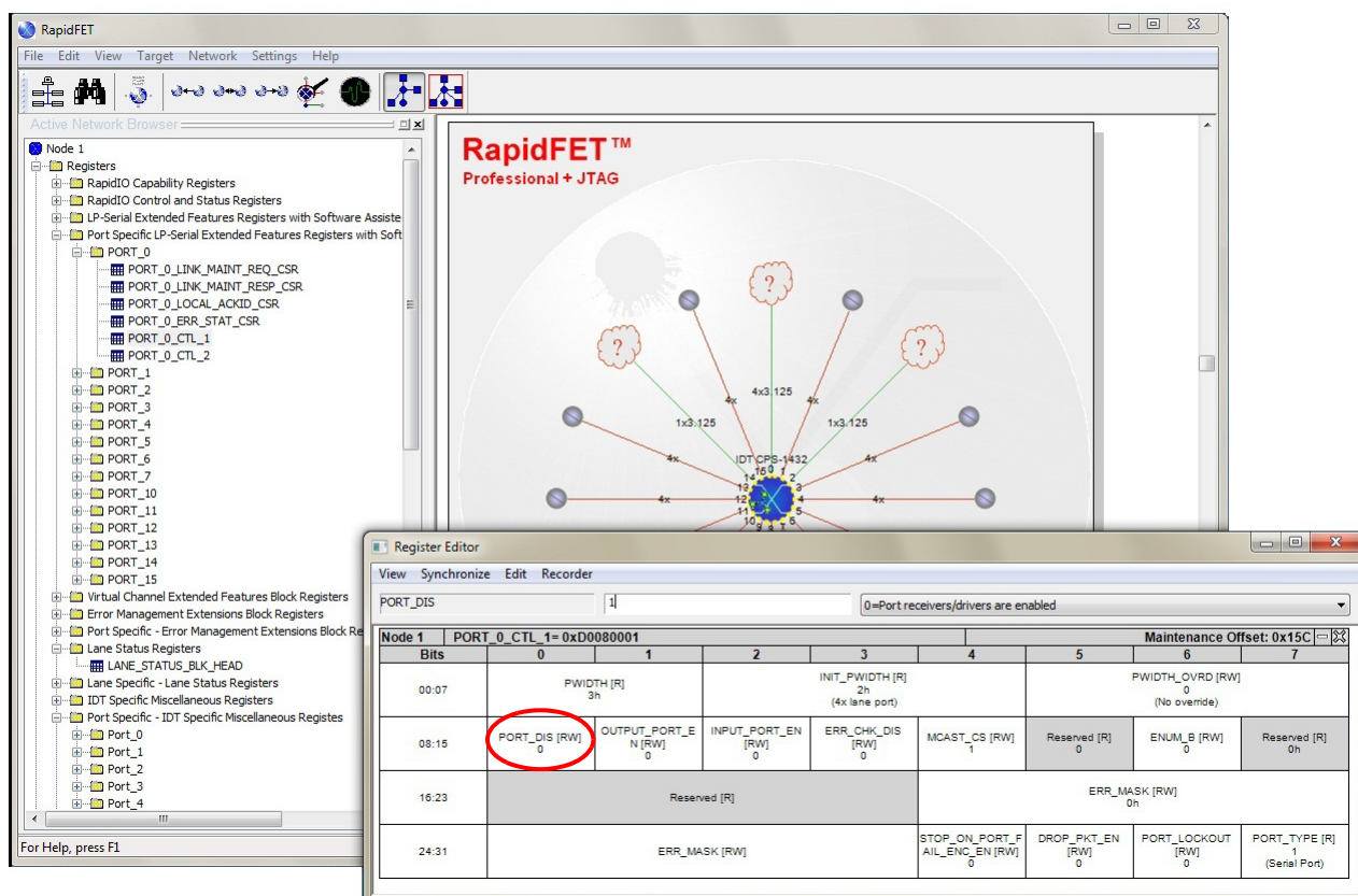
Figure 10: Register Editor – Disable Port
