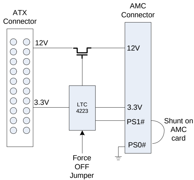
Figure 2: AMC Power Controller
