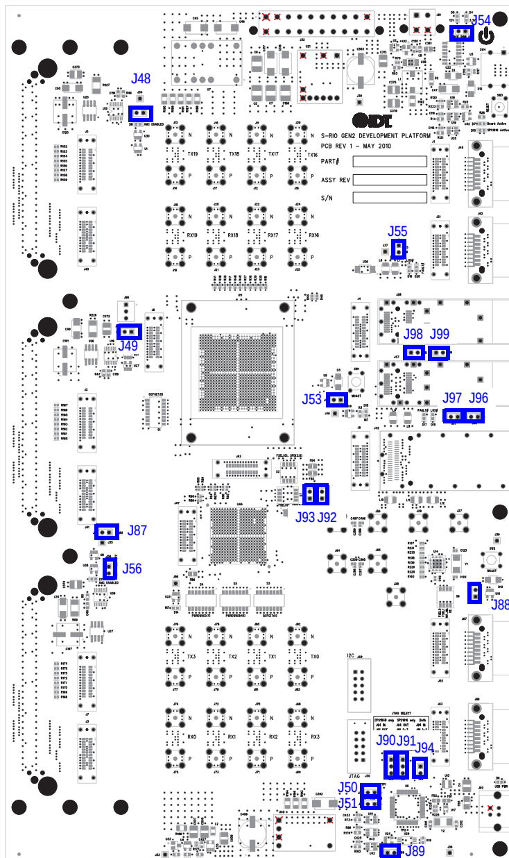
Figure 12: Jumper Locations
