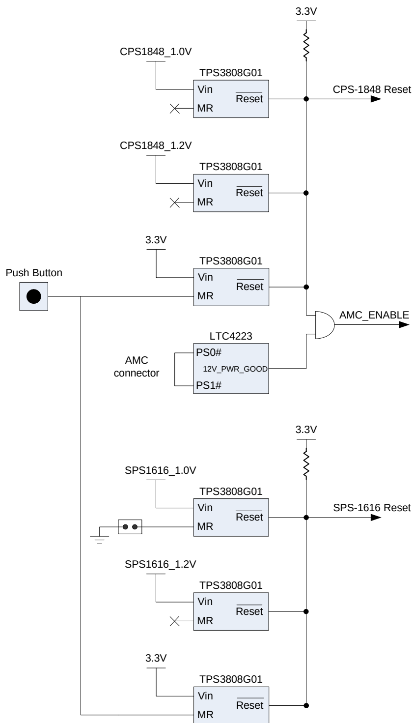
Figure 4: Board Reset
