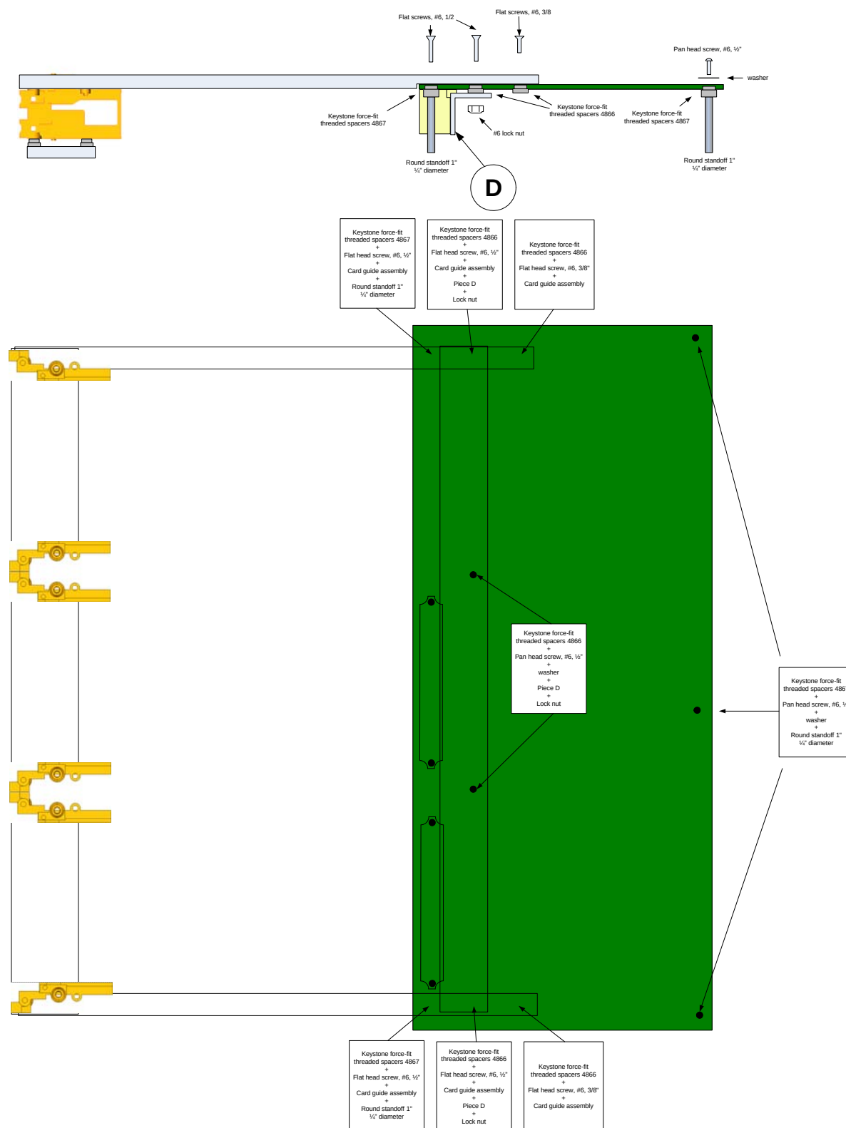
Figure 34: SRDP2 Mechanical Assembly
