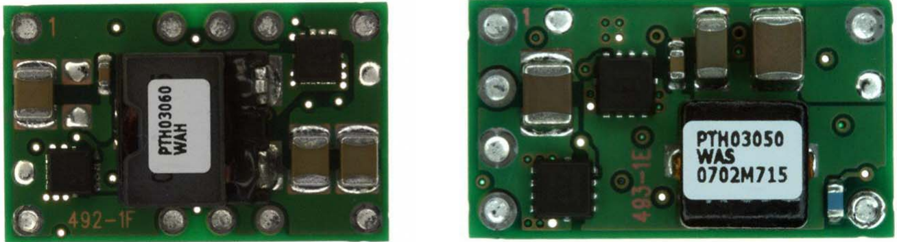
Figure 8: PTH03060W Module
