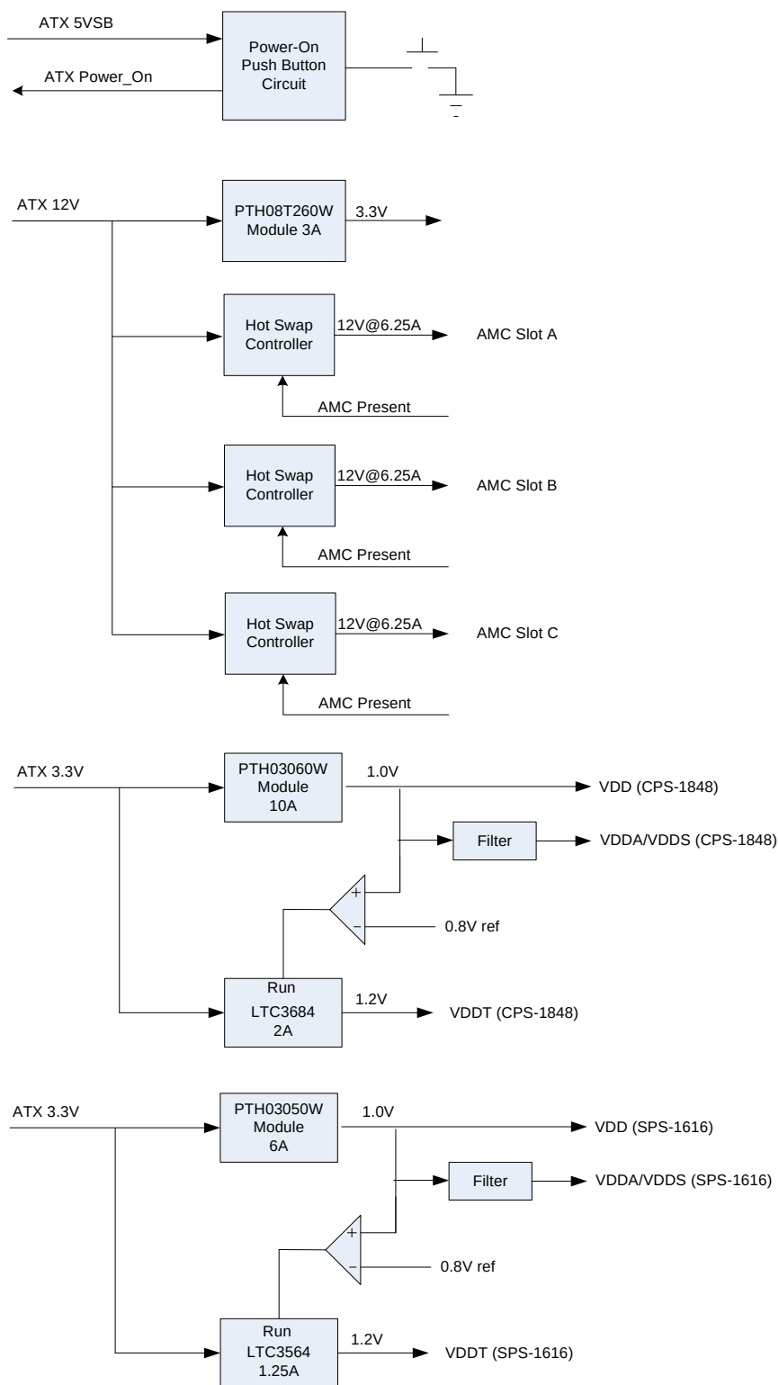
Figure 5: Power Distribution
