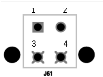
Figure 24: J61 - Optional 12V ATX Supply
