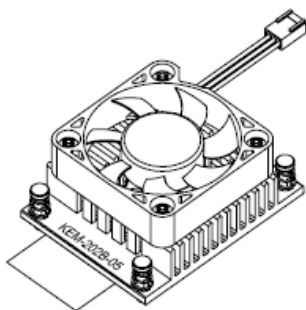
Figure 29: Heatsink with Fan Mounted on CPS-1848
