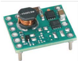
Figure 6: PTH08T260 Module
