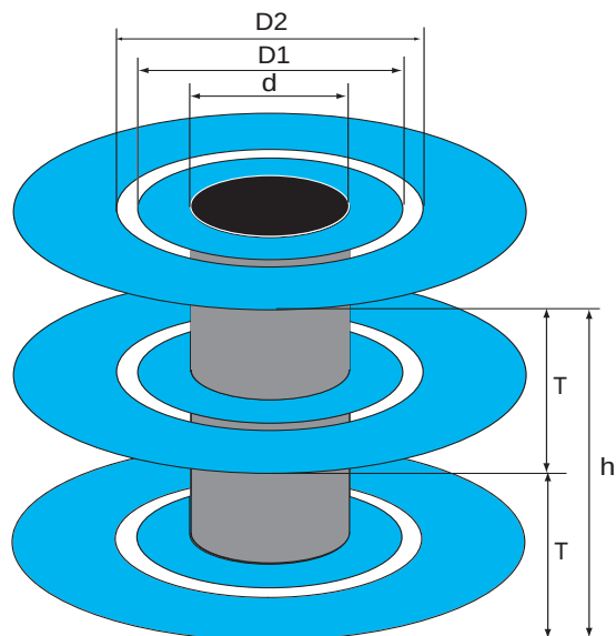
Figure 16: Via Construction
