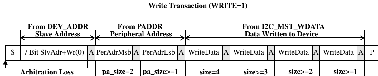
Figure 32: Software-initiated Master Transactions
