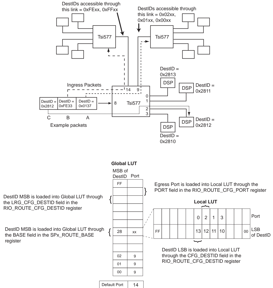
Figure 10: Hierarchical Mode Routing Example
