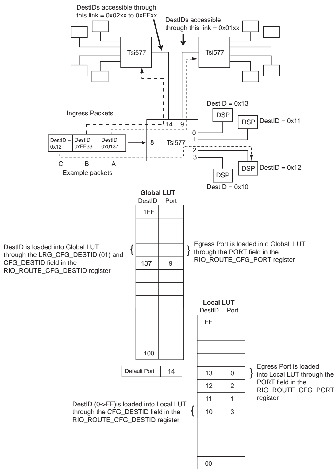
Figure 7: Flat Mode Routing Example
