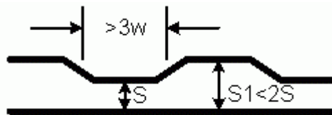
Figure 24: Differential Skew Matching Serpentine
