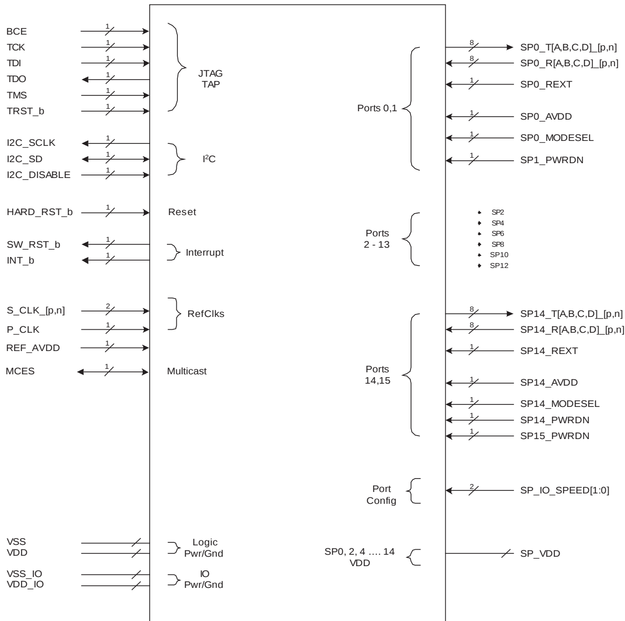
Figure 1: Signal Groupings
