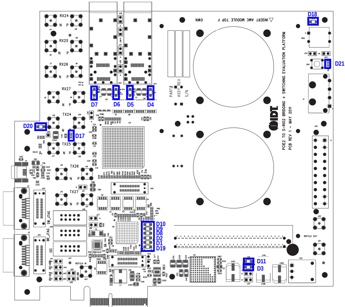
Figure 19: LED Locations
