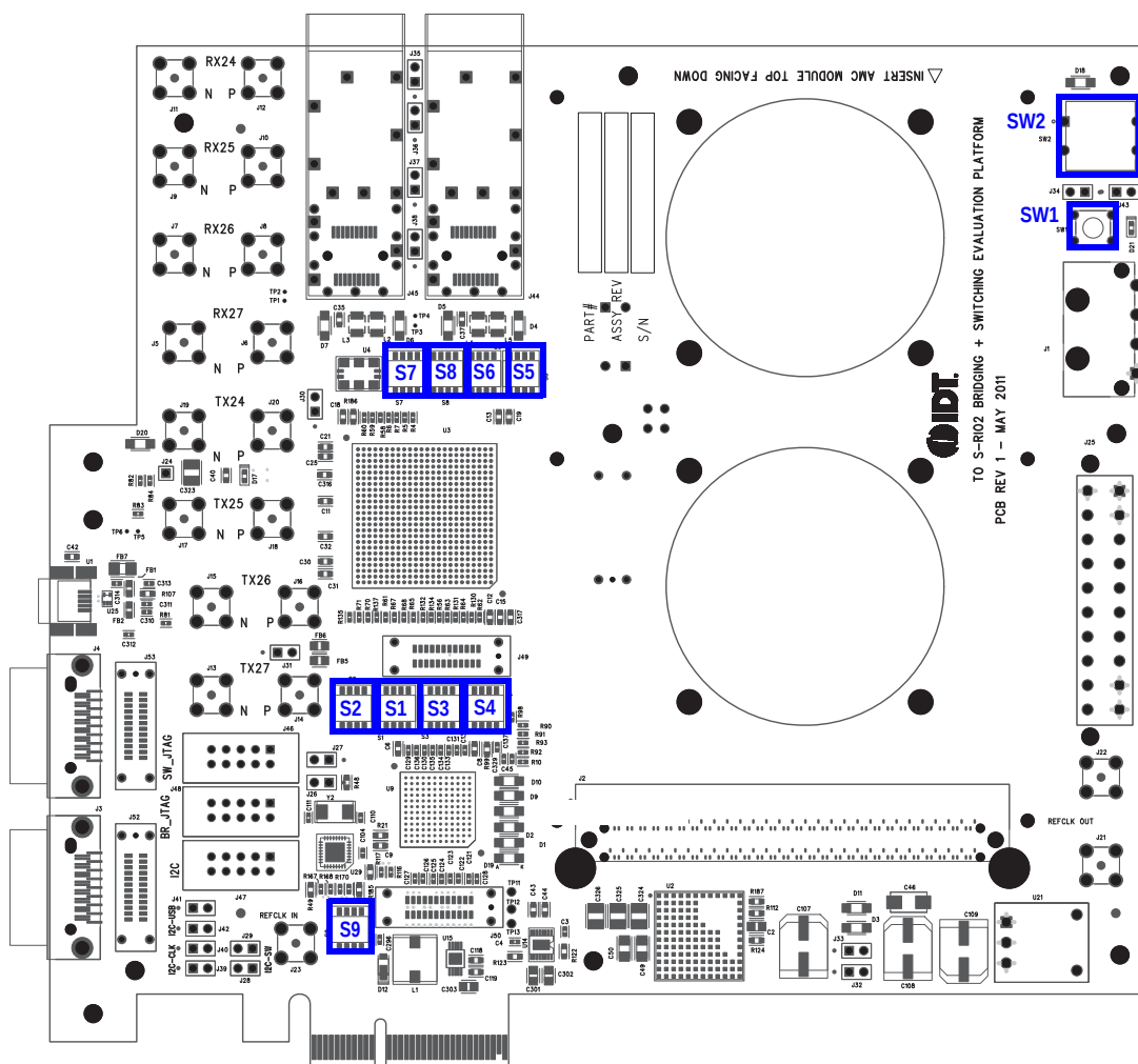
Figure 14: Switch Locations
