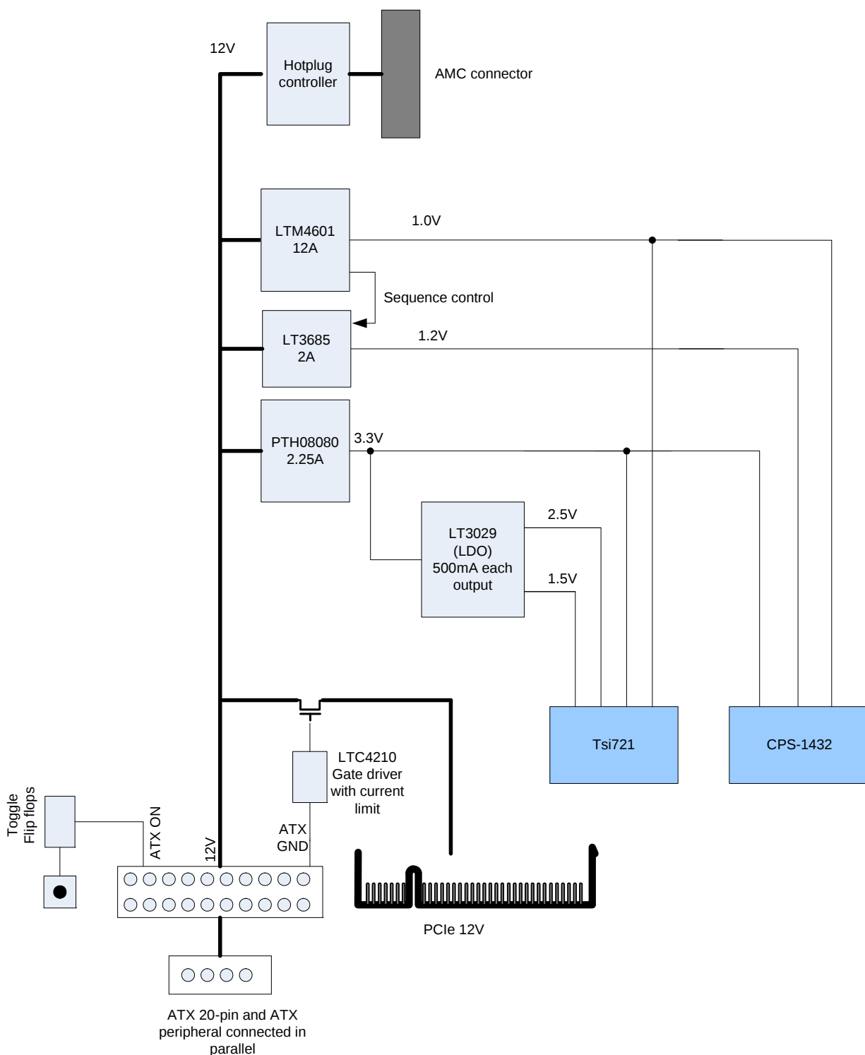
Figure 10: Voltage Regulators
