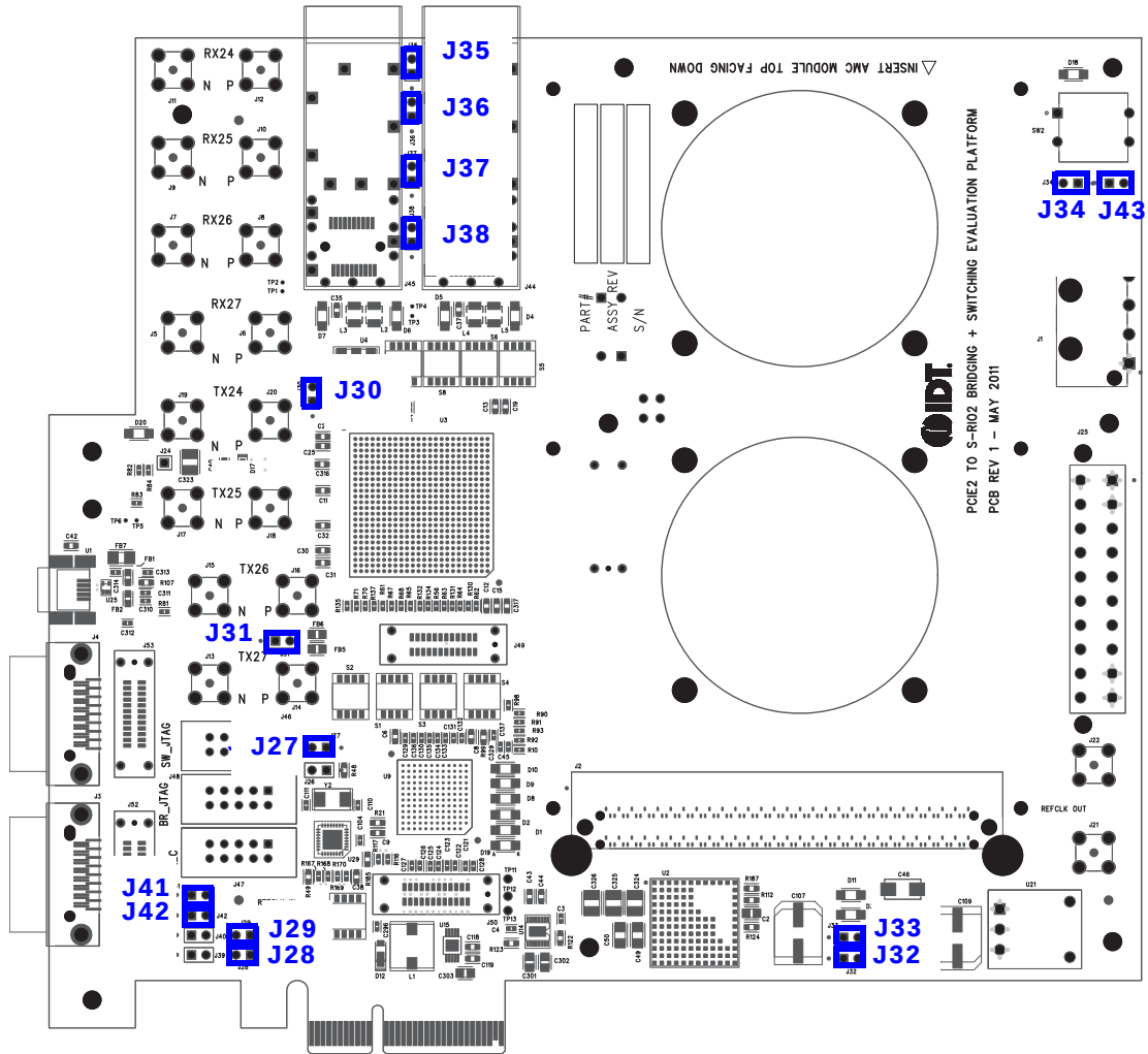
Figure 17: Jumper Locations
