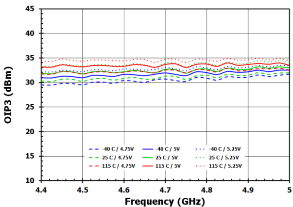
Figure 37. OIP3
