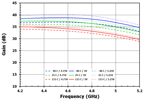
Figure 33. Gain
