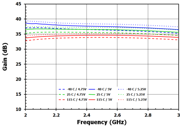
Figure 3. Gain
