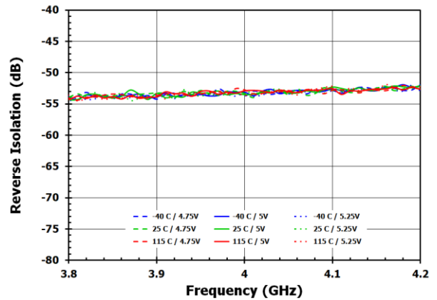
Figure 24. Reverse Isolation
