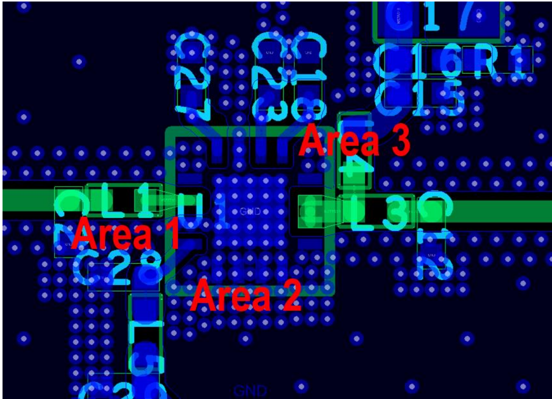
Figure 48. Layout Example
