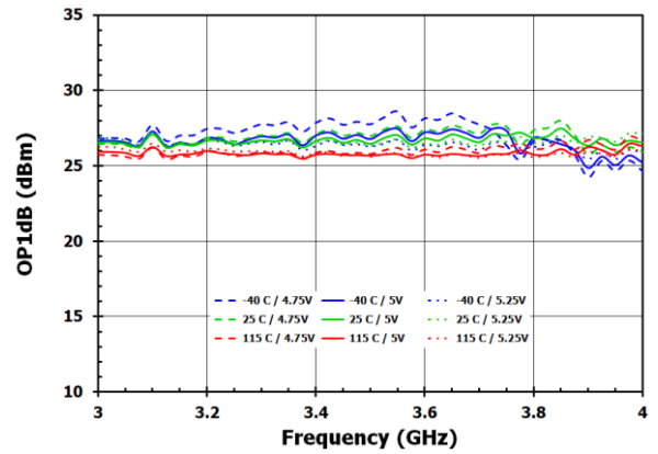
Figure 18. OP1dB
