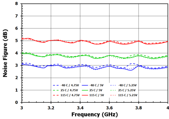
Figure 21. Noise Figure
