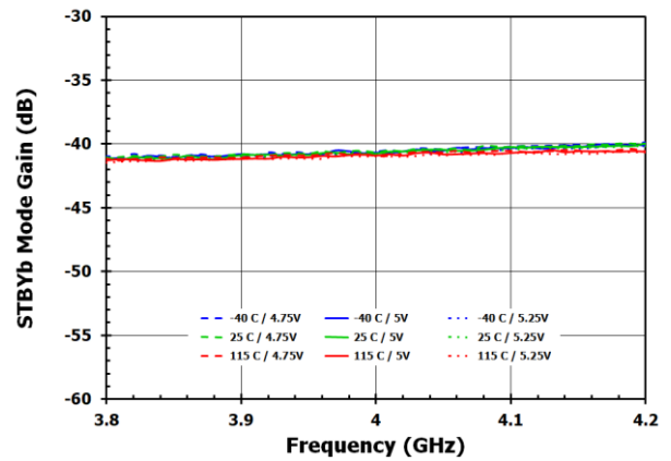
Figure 32. STBYb Gain
