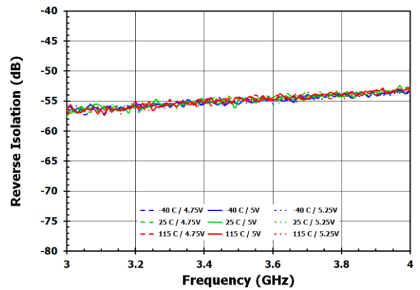
Figure 14. Reverse Isolation
