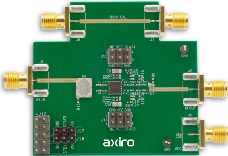
Figure 12. Top View
