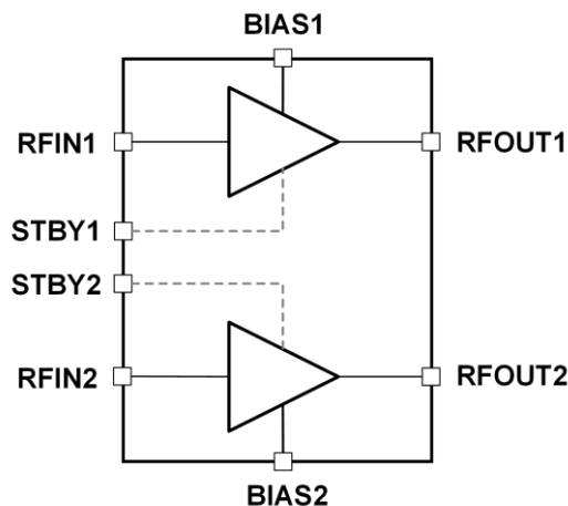
Figure 1. Block Diagram
