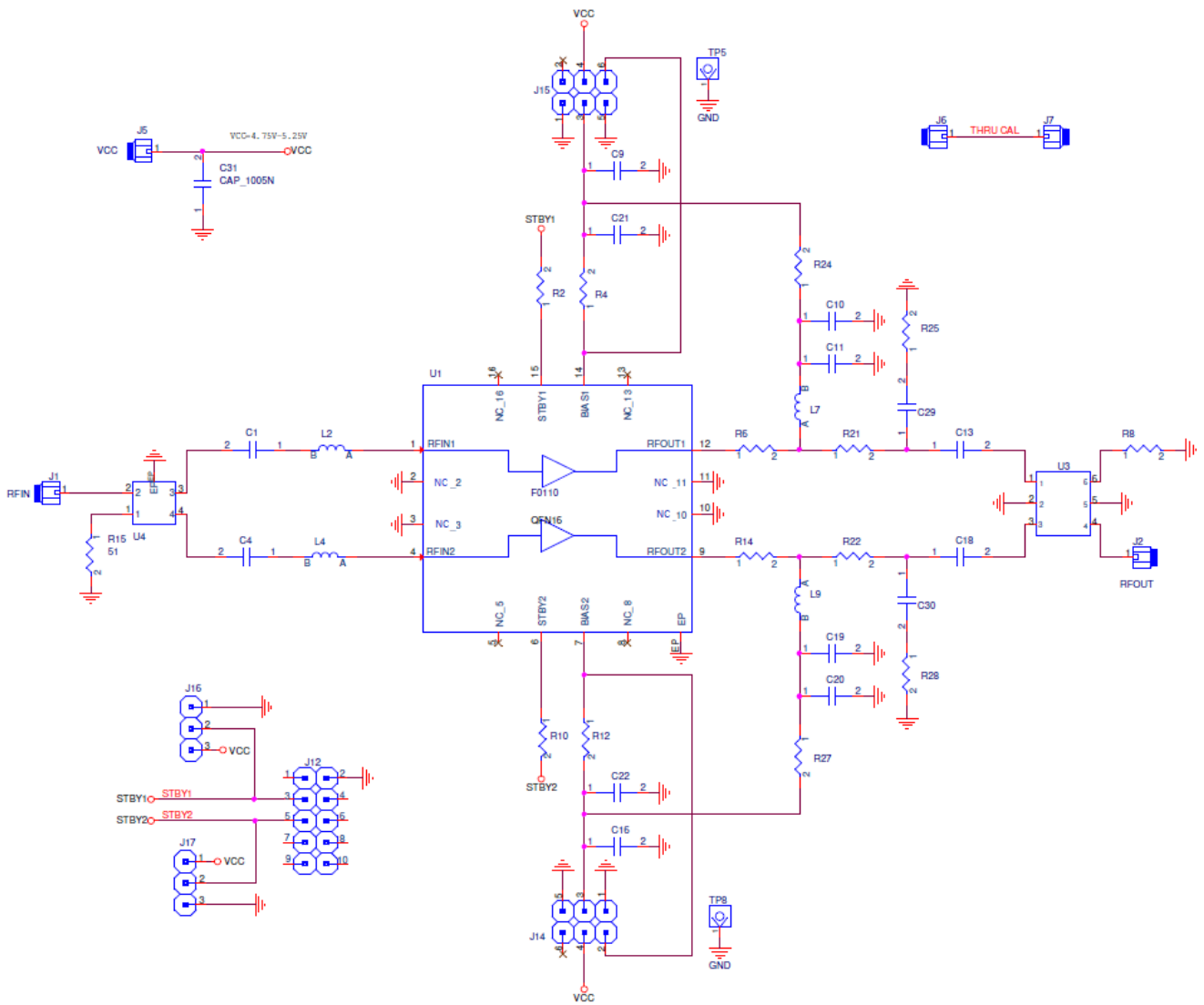
Figure 14. Electrical Schematic
