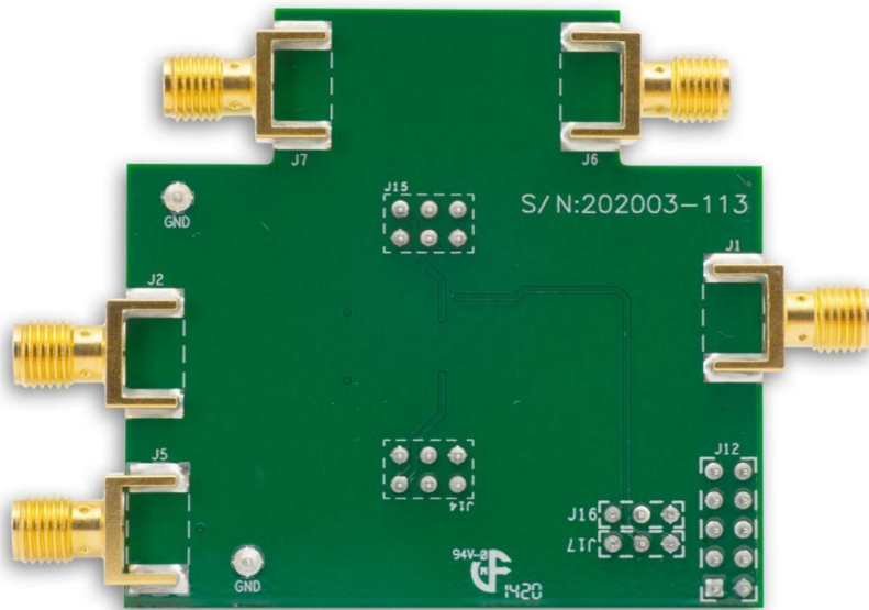
Figure 13. Bottom View
