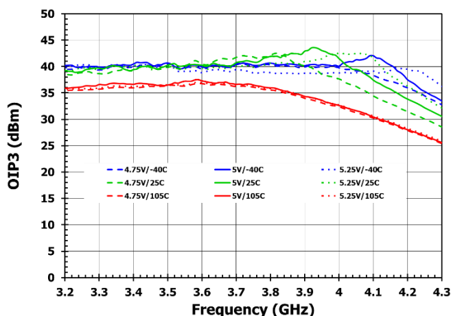
Figure 21. OIP3
