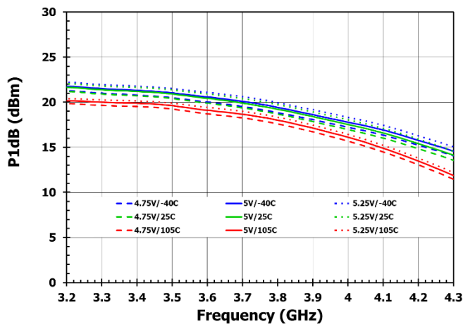
Figure 19. OP1dB
