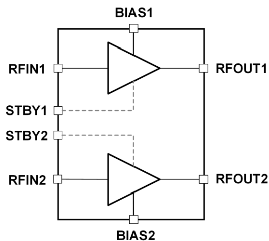
Figure 1. Block Diagram
