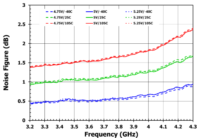
Figure 17. Noise Figure
