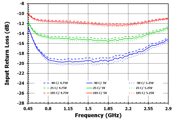
Figure 56. S11, DSA2 = 25dB, Bypass OFF
