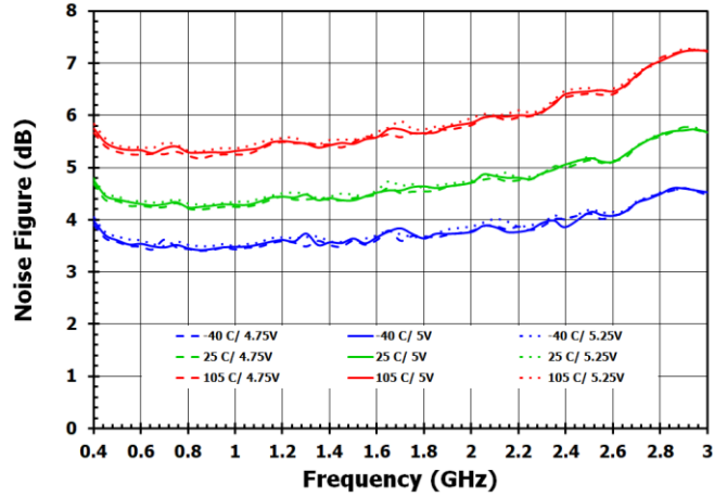
Figure 90. Noise Figure, DSA2 = 25dB, Bypass OFF
