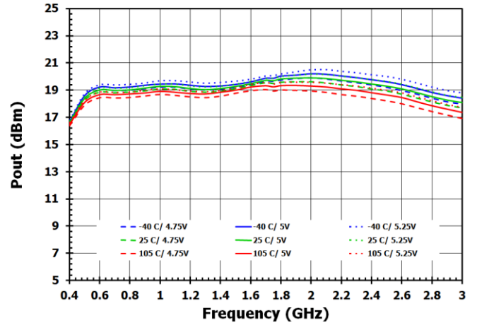
Figure 96. OP1dB at DSA2 = 15dB, Bypass OFF
