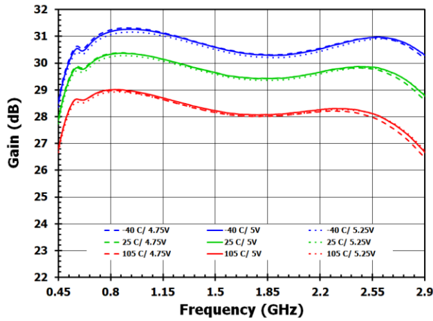
Figure 5. Gain, DSA0 = 6dB, Bypass OFF
