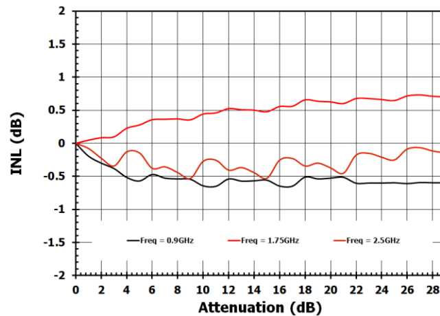
Figure 36. DSA2 INL (Absolute Attenuation Error) Bypass ON
