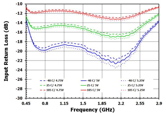
Figure 50. S11, DSA2 = 5dB, Bypass OFF
