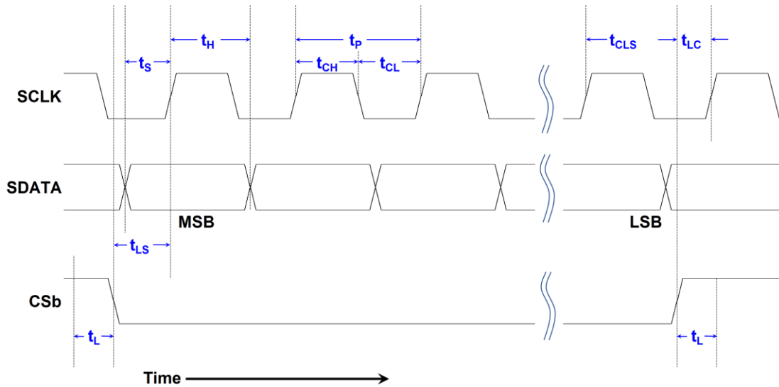
Figure 108. SPI Serial Register Timing Diagram
