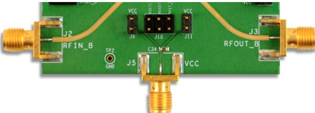
Figure 121. Power Supply and Logic Voltage Connections
