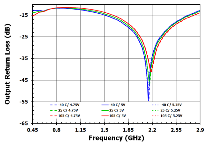
Figure 78. S22, DSA3 = 6dB, Bypass OFF
