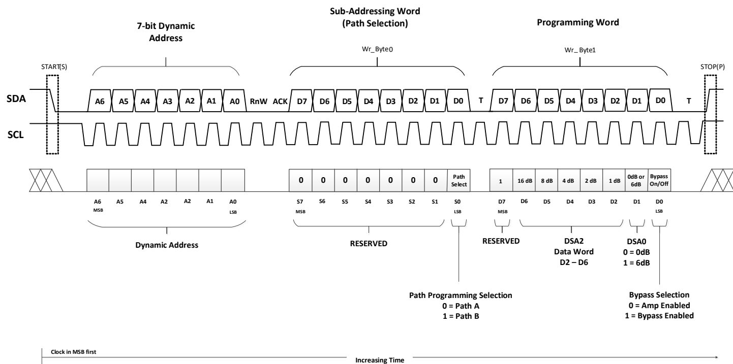
Figure 112. I3C Timing Diagram
