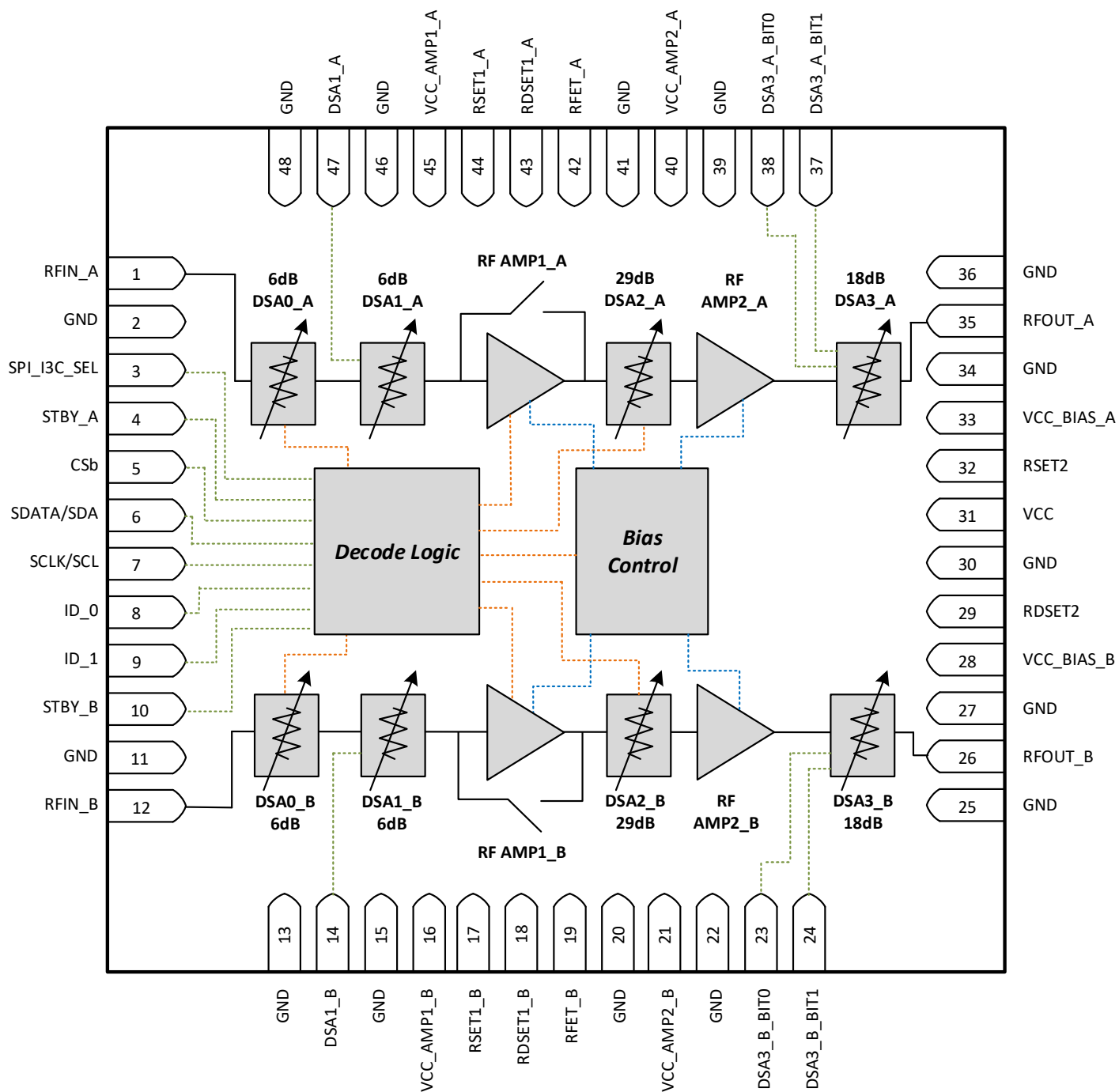
Figure 2. Pin Assignments for 7 × 7 × 0.75 mm 48-LGA Package – Top View
