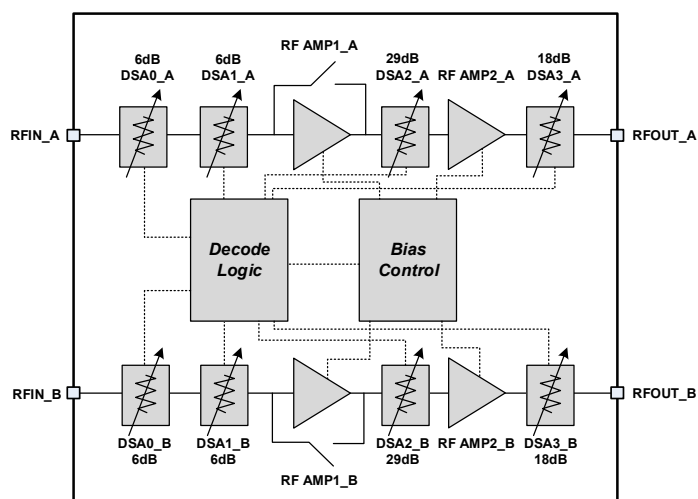
Figure 1. Block Diagram
