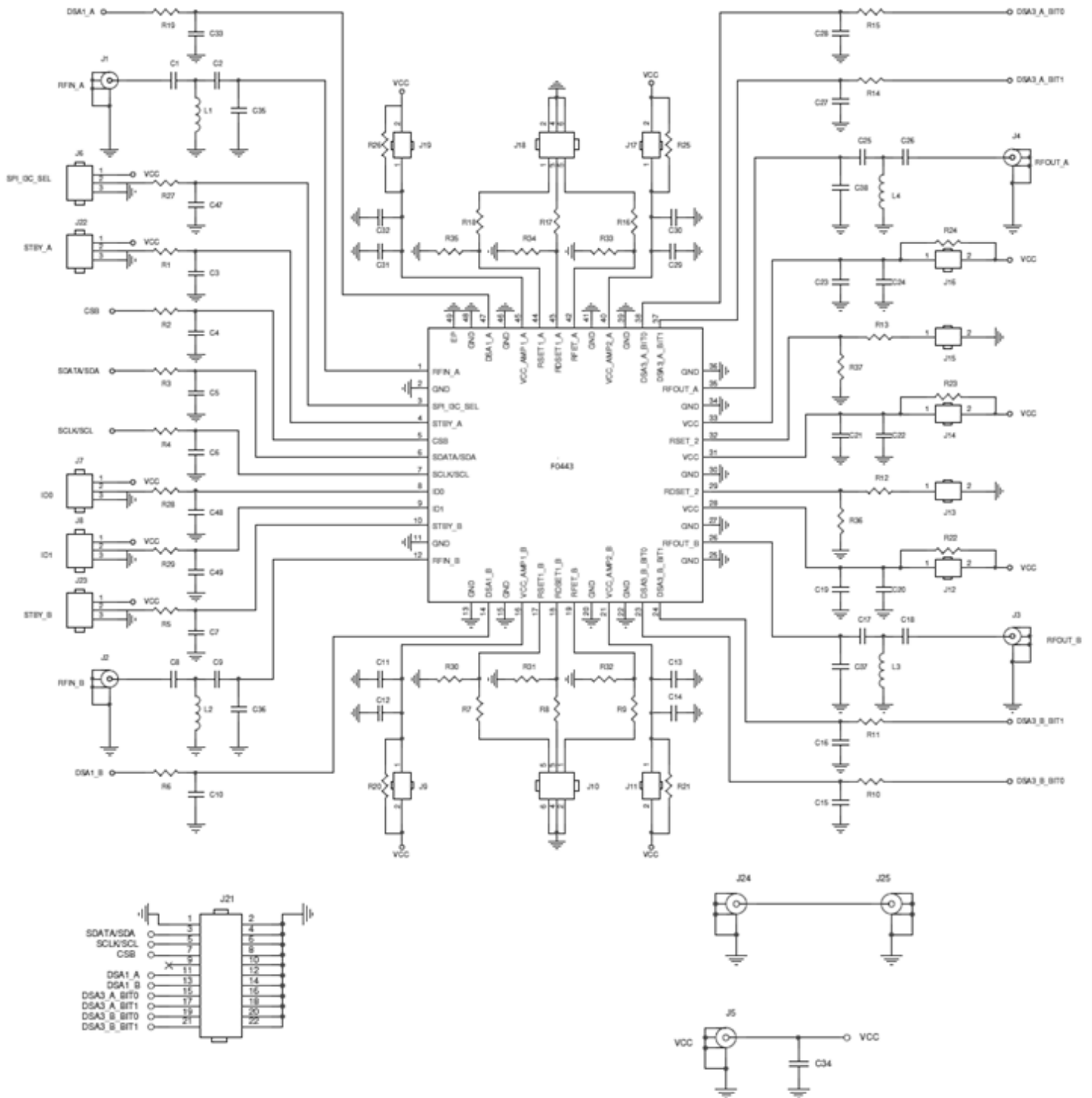
Figure 120. Electrical Schematic
