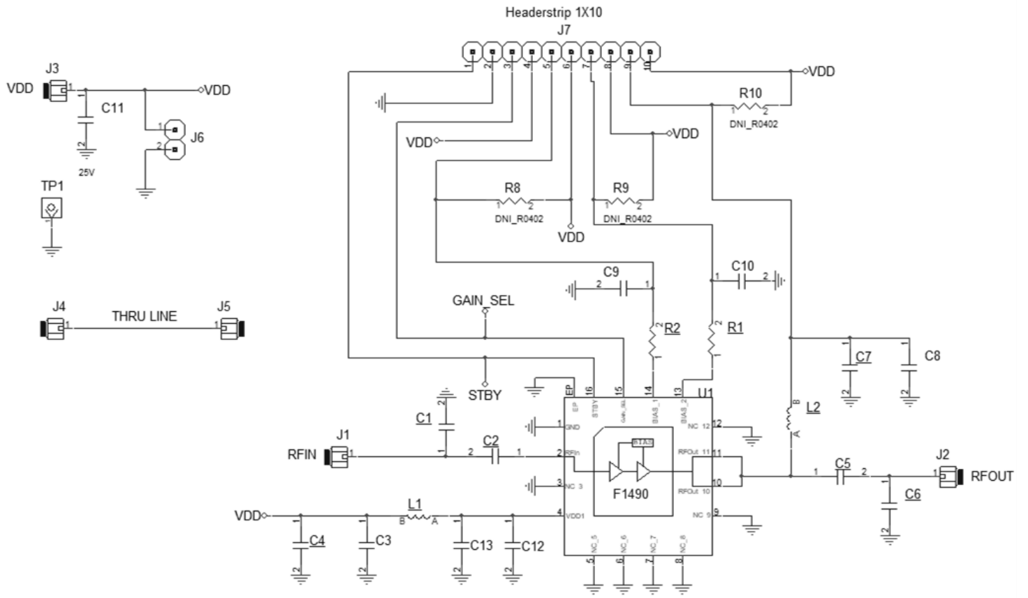
Figure 94. Electrical Schematic
