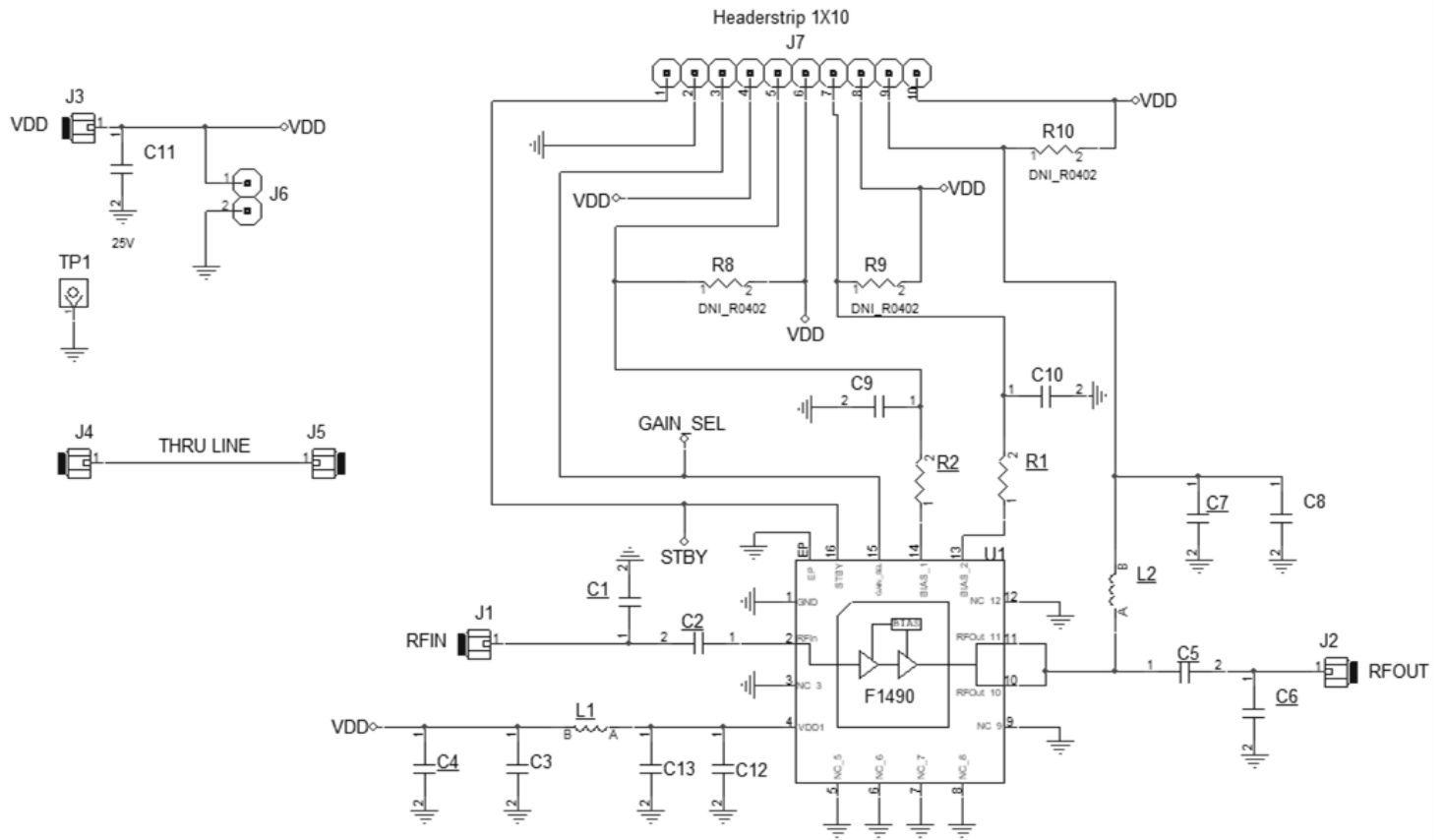
Figure 94. Electrical Schematic
