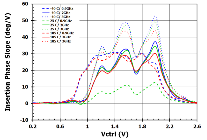
Figure 9. Insertion Phase Slope
