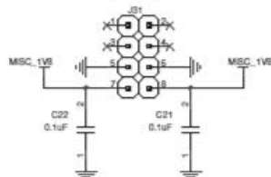
F2232H SPI MODULE (REVC) CONNECTOR 2 (2x4)
