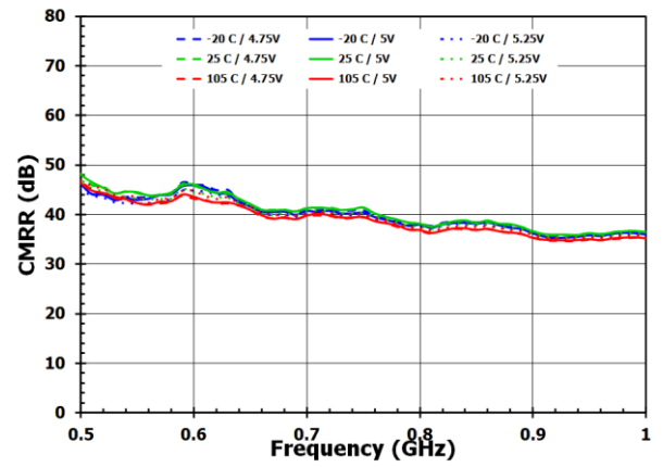
Figure 8. CMRR
