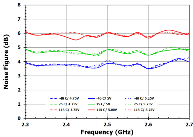
Figure 11. Noise Figure
