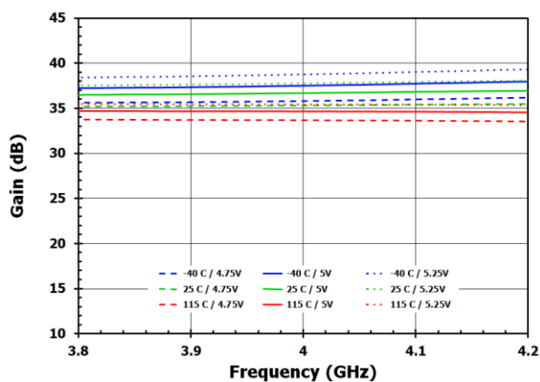
Figure 23. Gain
