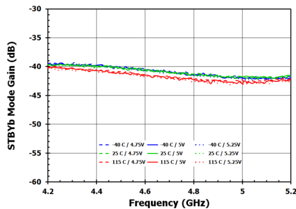
Figure 42. STBYb Gain
