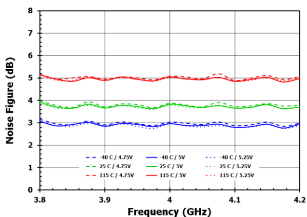
Figure 31. Noise Figure
