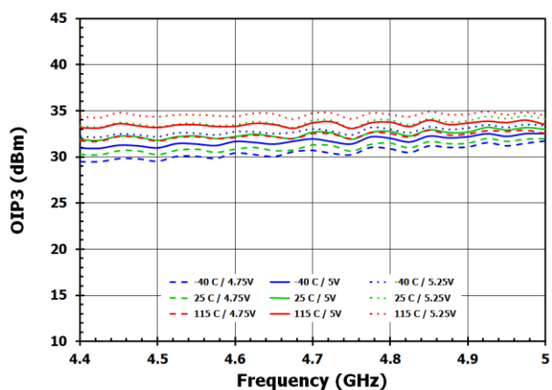
Figure 37. OIP3
