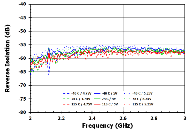
Figure 4. Reverse Isolation
