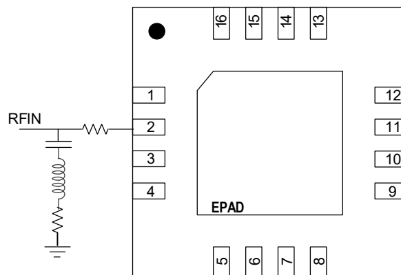
Figure 47. Recommended RF Input Circuit Implementation for Large-Signal Linearity Optimization – 3600MHz to 4200MHz Range
