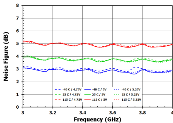
Figure 21. Noise Figure
