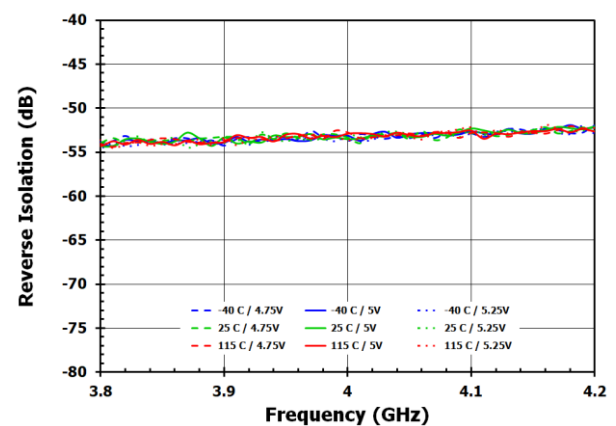
Figure 24. Reverse Isolation
