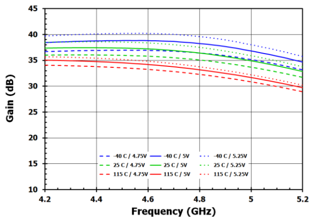
Figure 33. Gain
