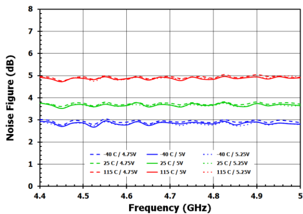
Figure 41. Noise Figure
