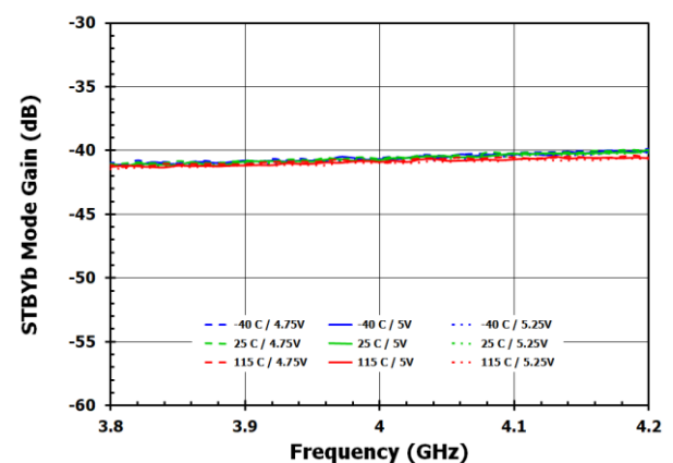
Figure 32. STBYb Gain
