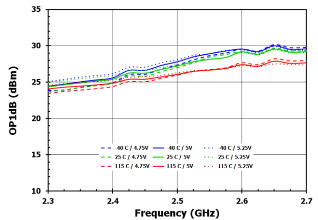
Figure 8. OP1dB
