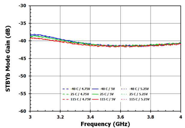
Figure 22. STBYb Gain
