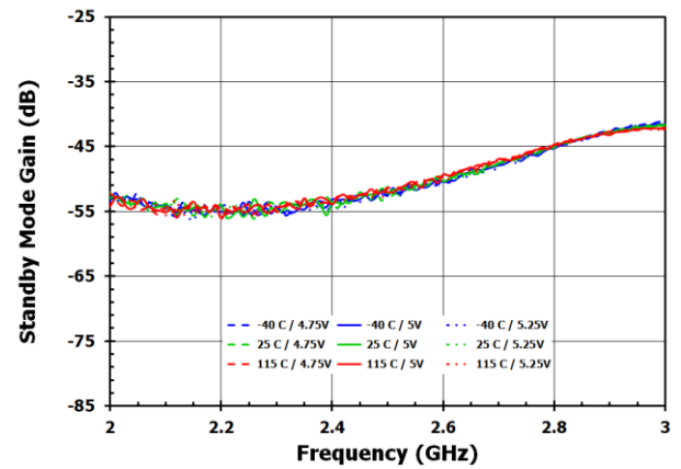
Figure 12. STBYb Gain
