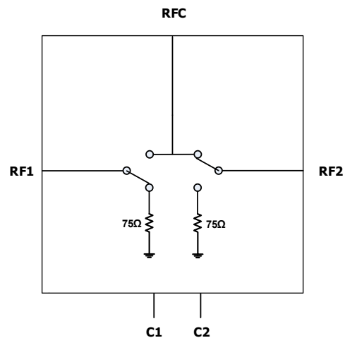
Figure 1. Block Diagram
