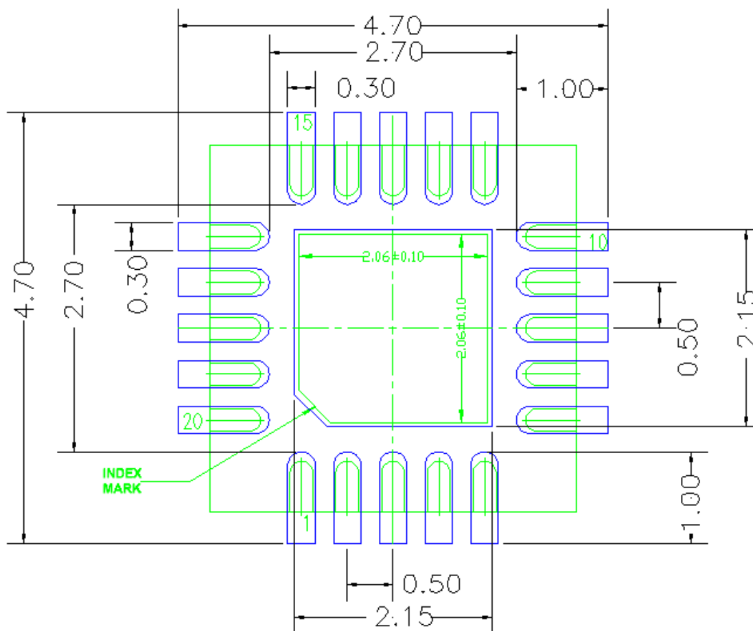
Figure 31. Recommended Land Pattern
