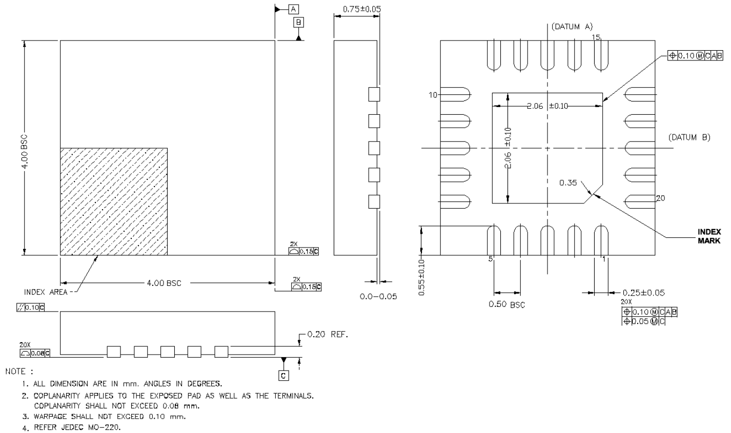
Figure 30. Package Outline Drawing
