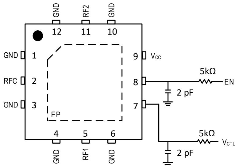
Figure 16. Control Pin Interface Schematic
