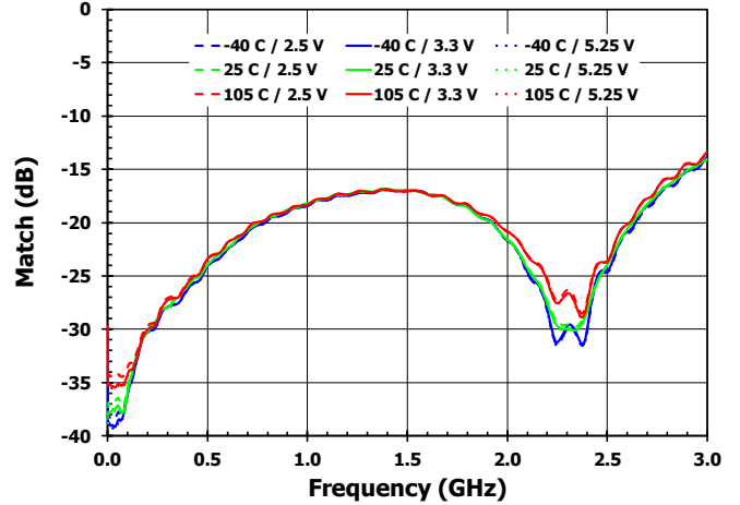
Figure 13. RF2 Return Loss [RF2 On State]
