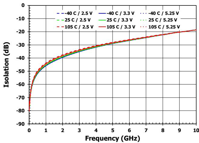
Figure 19. RF1 to RF2 Isolation [RF2 On State]
