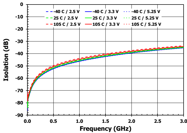
Figure 9. RF1 to RF2 Isolation [RF2 On State]
