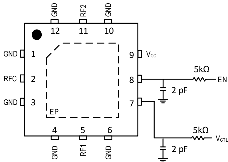
Figure 26. Control Pin Interface Schematic
