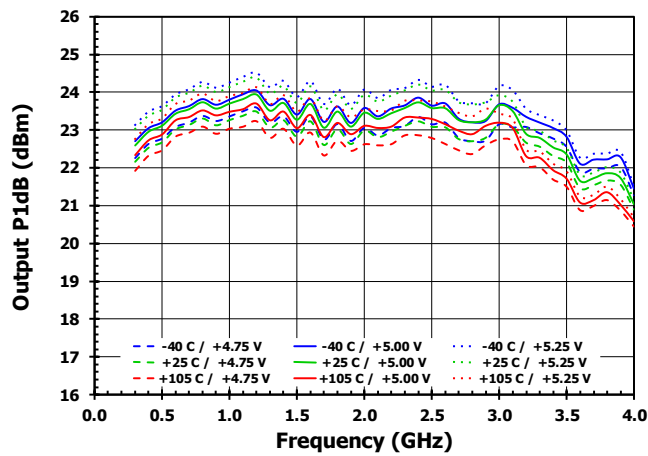
Figure 19. Output P1dB versus Frequency [Attenuation = 0dB]
