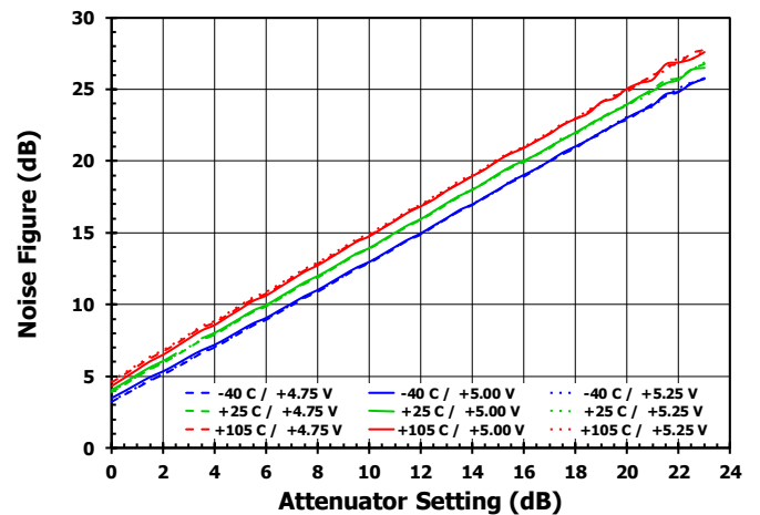
Figure 32. Noise Figure versus Attenuation [2.0GHz]
