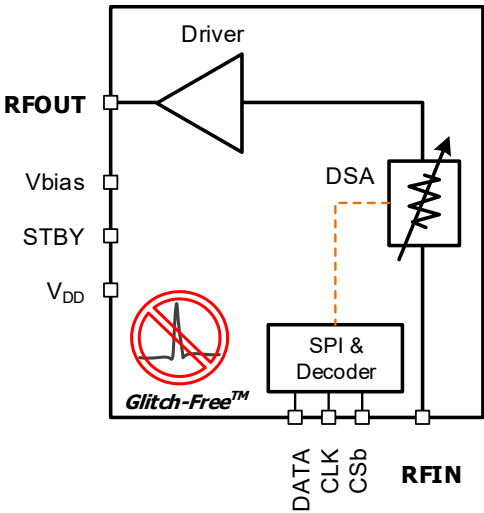
Figure 1. Block Diagram
