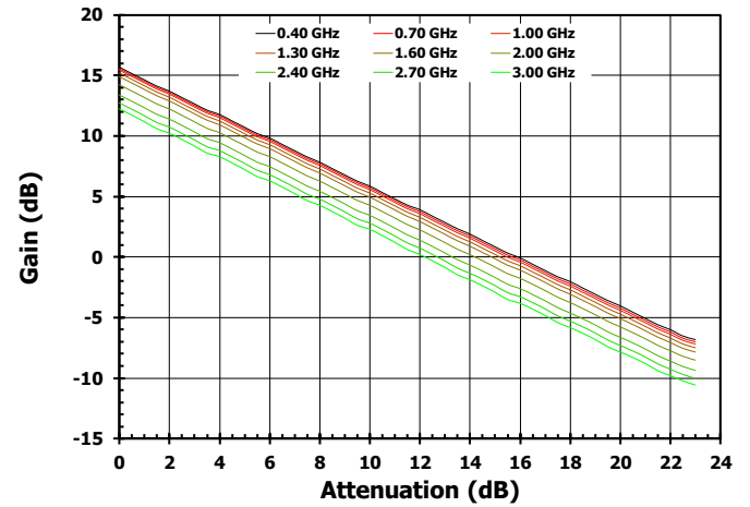
Figure 6. Gain versus Attenuation [+25°C]
