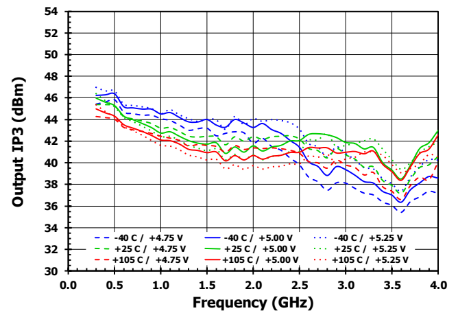
Figure 20. Output IP3 versus Frequency [Attenuation = 0dB]
