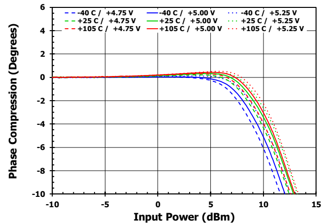
Figure 30. Phase Compression versus Input Power [2.7GHz, Attenuation = 0dB]
