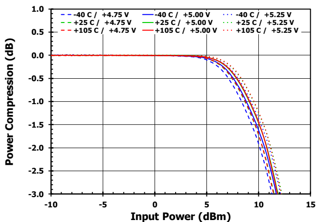
Figure 25. Compression versus Input Power [0.7GHz, Attenuation = 0dB]
