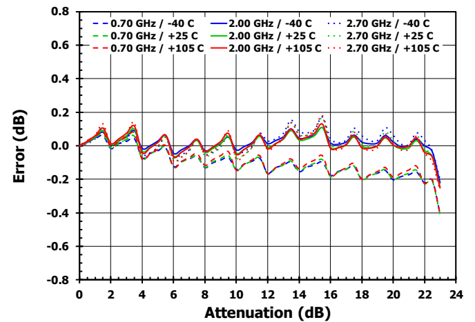
Figure 16. Attenuator Accuracy versus Attenuation
