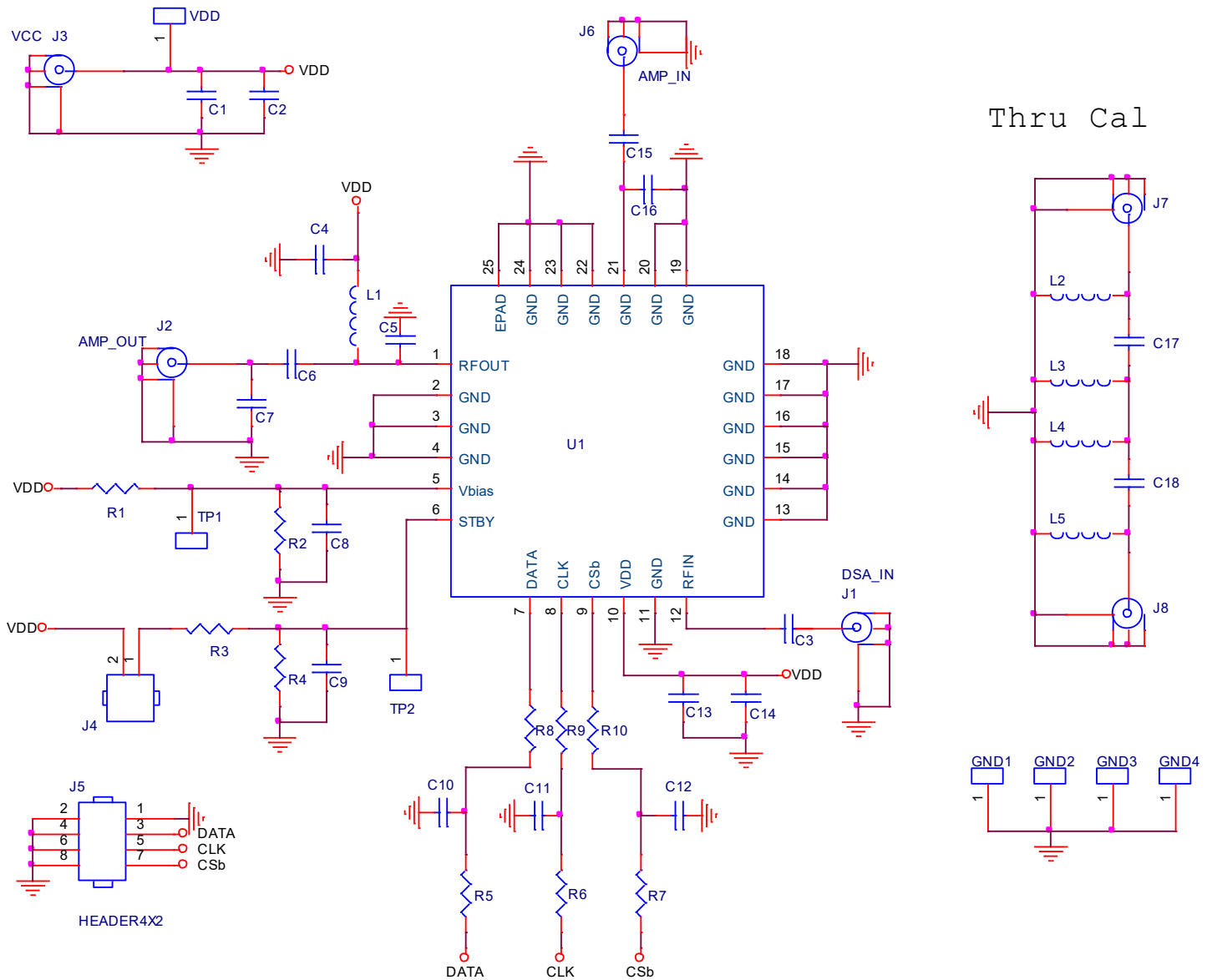
Figure 41. Electrical Schematic
