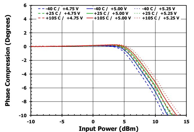
Figure 26. Phase Compression versus Input Power [0.7GHz, Attenuation = 0dB]
