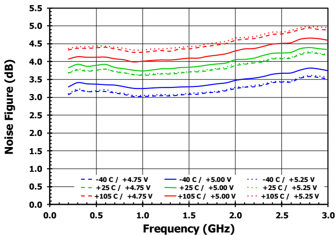
Figure 31. Noise Figure versus Frequency [Attenuation = 0dB]
