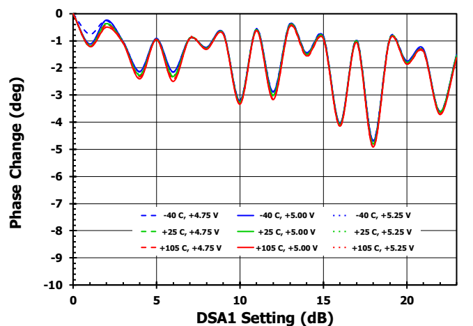
Figure 17. Phase Deviation Between Adjacent States vs. DSA1 Setting (3.6GHz)
