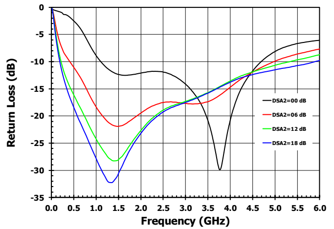
Figure 13. Output Return Loss for DSA2 Settings
