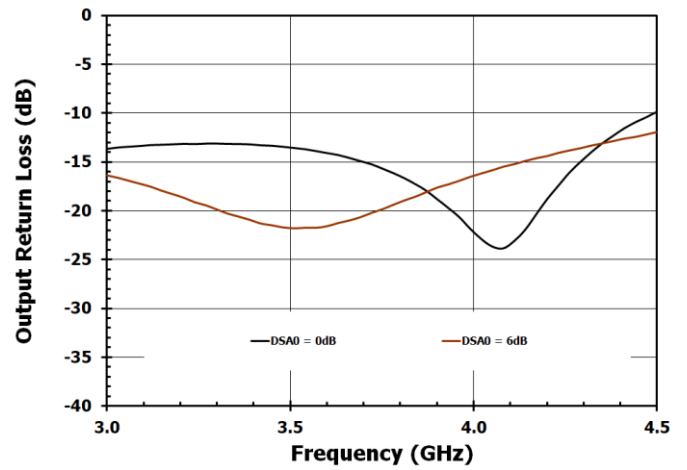
Figure 44. Output Return Loss for DSA0 Settings
