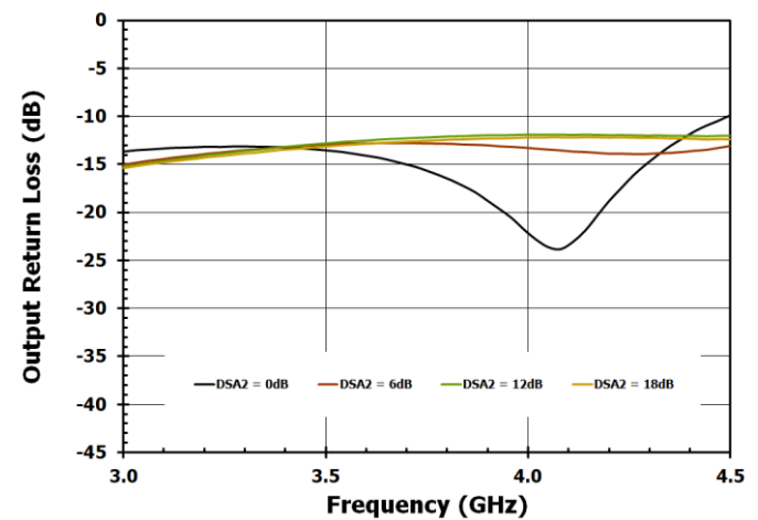
Figure 48. Output Return Loss for DSA2 Settings
