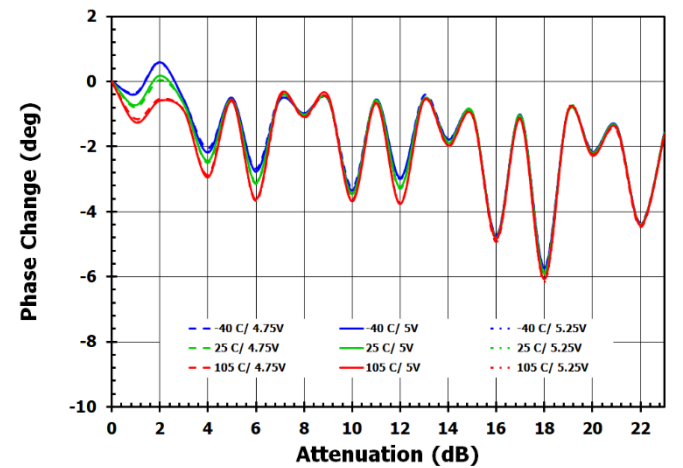
Figure 52. Phase Deviation Between Adjacent States vs. DSA1 Setting (4GHz)
