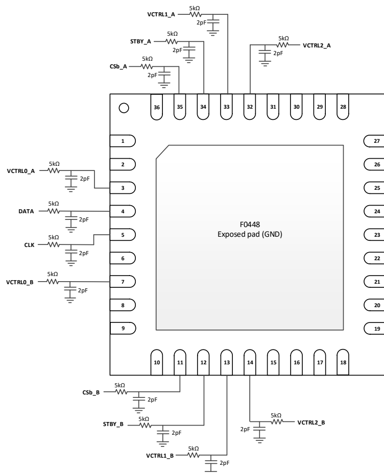
Figure 82. Control Pin Interface
