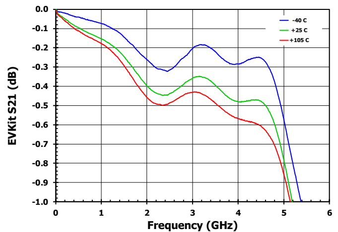
Figure 36. EVKit Connector and Trace Losses
