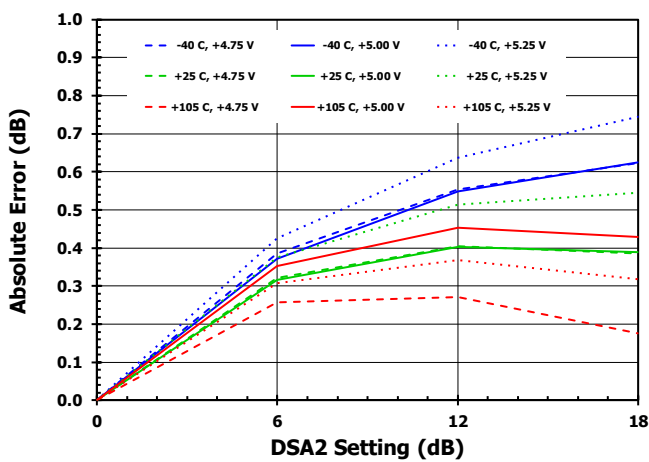
Figure 24. DSA2 Absolute Attenuation Error (INL) at 3.6GHz
