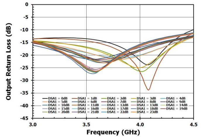
Figure 46. Output Return Loss for DSA1 Settings
