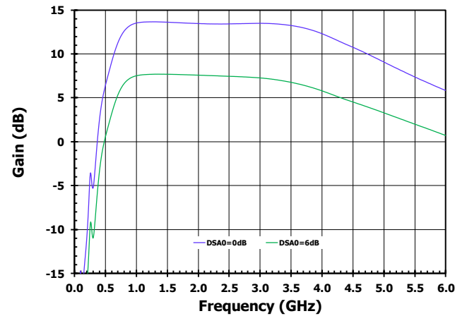
Figure 4. Gain vs. Frequency for DSA0 Settings
