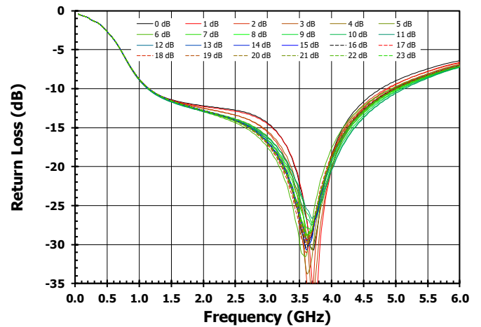
Figure 11. Output Return Loss for DSA1 Settings
