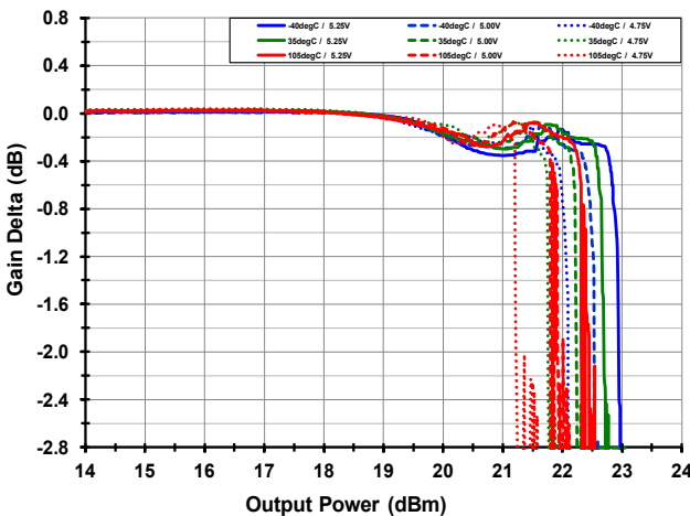
Gain Compression [900 MHz]
