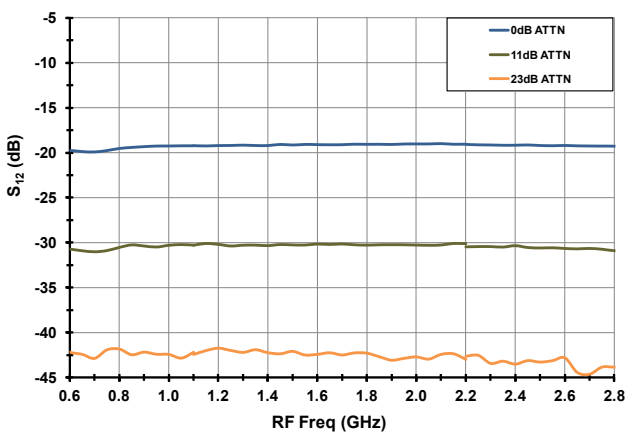
S12 (device+C5 cap) [ T_{AMB} = 25^{\circ}C , V_{CC} = 5.00 Volts]
