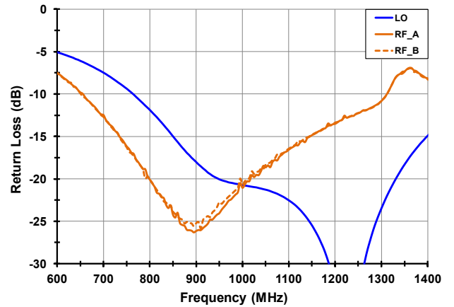
EVkit RF & LO Port Match (T A = 25C)
