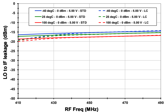
LO to IF Leakage vs. T CASE (130 MHz IF)
