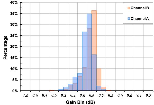
Gain Distribution ( F_{RF} = 915\text{ MHz} , LC mode, N = 1598 )
