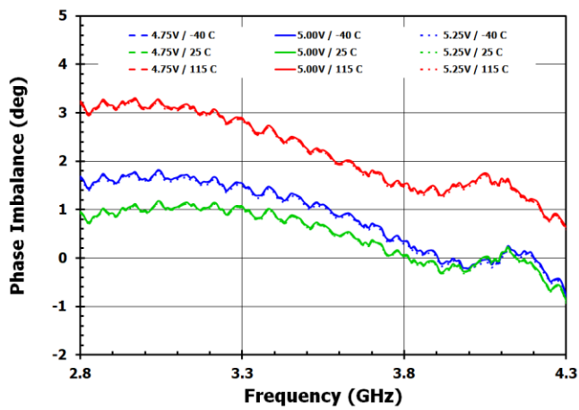
Figure 11. Phase Imbalance
