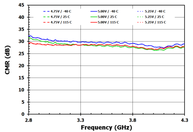
Figure 12. CMR
