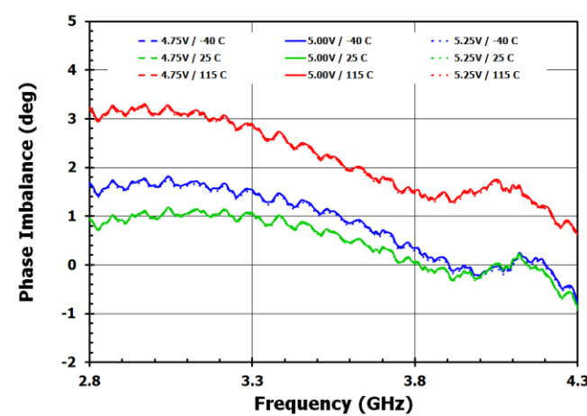
Figure 11. Phase Imbalance
