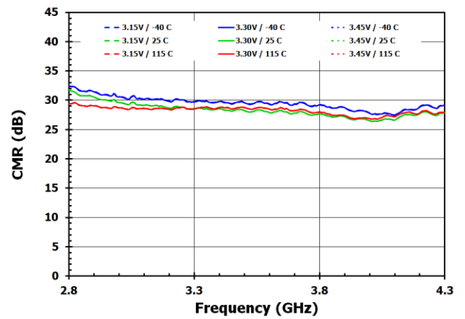
Figure 22. CMR
