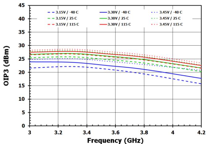
Figure 17. Output IP3
