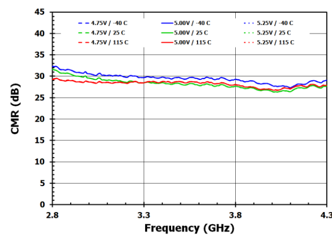
Figure 12. CMR
