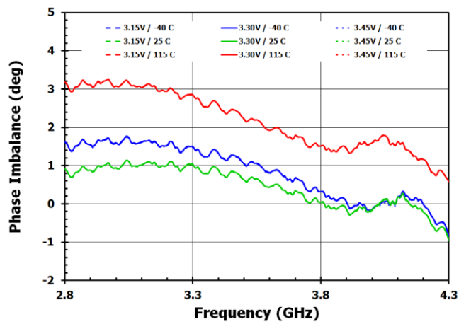
Figure 21. Phase Imbalance
