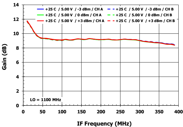
IF Gain flatness vs. LO Power [ G_{MIXR\_Tr} HS injection]
