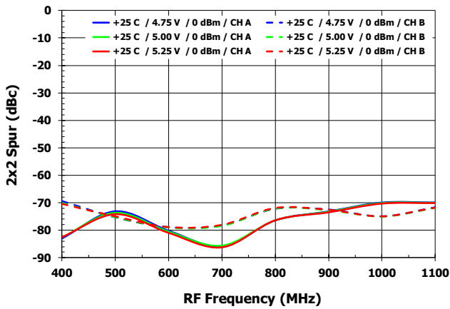
2x2 Rejection vs. V_{cc} [ 2x2_{MIXR} , HS rejection]
