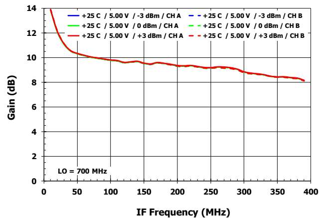
IF Gain flatness vs. LO Power [ G_{MIXR\_Tr} LS injection]
