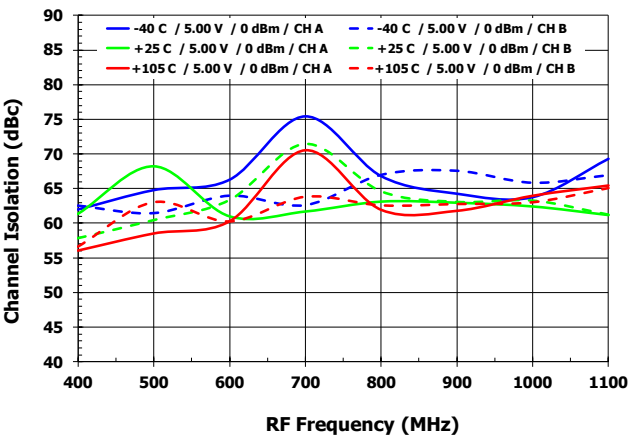
Channel Isolation vs. T_{case} [ISO IFr , HS injection]
