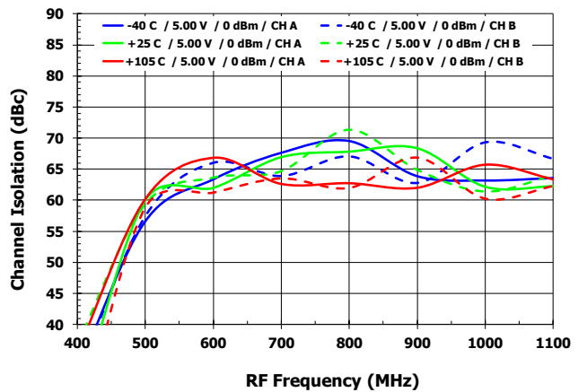
Channel Isolation vs. T_{case} [ISO IFr , LS injection]
