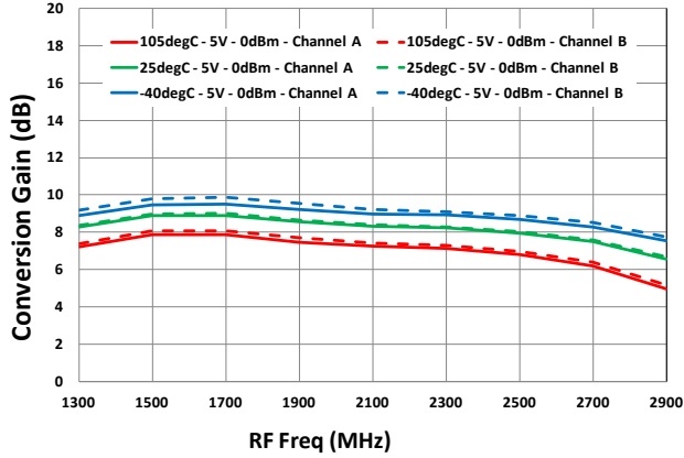
Gain vs. T_{case} [ G_{MIXR} , HS Injection]
