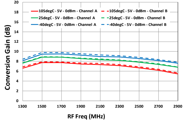
Gain vs. T_{case} [ G_{MIXR} , LS Injection]
