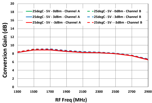
Gain vs. LO Power [ G_{MIXR} , HS Injection]
