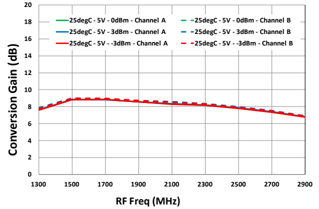
Gain vs. LO Power [ G_{MIXR} , LS Injection]
