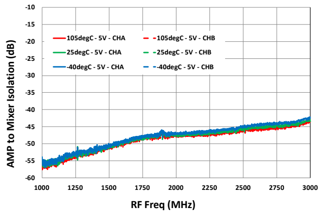
RF Amplifier to Mixer Isolation
