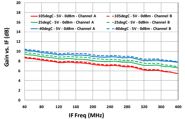
IF Gain flatness vs. T_{case} [ G_{MXR\_Tr} LS injection]
