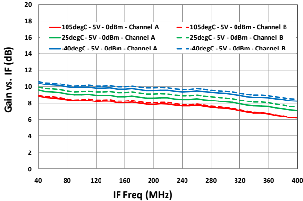
IF Gain flatness vs. T_{case} [ G_{MXR\_Tr} HS injection]
