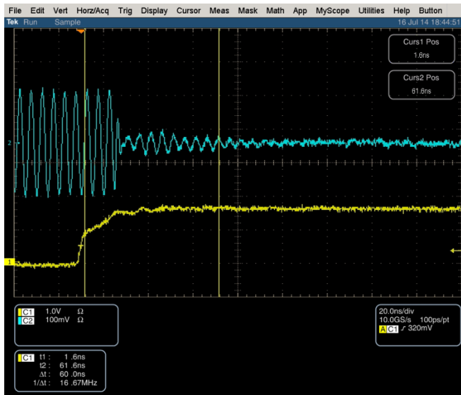
Mixer STBY OFF time [Max to Min, \tau_{MXR\_SET} ]
