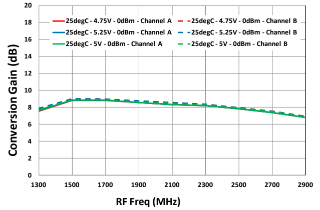
Gain vs. V_{cc} [ G_{MXR} , LS Injection]
